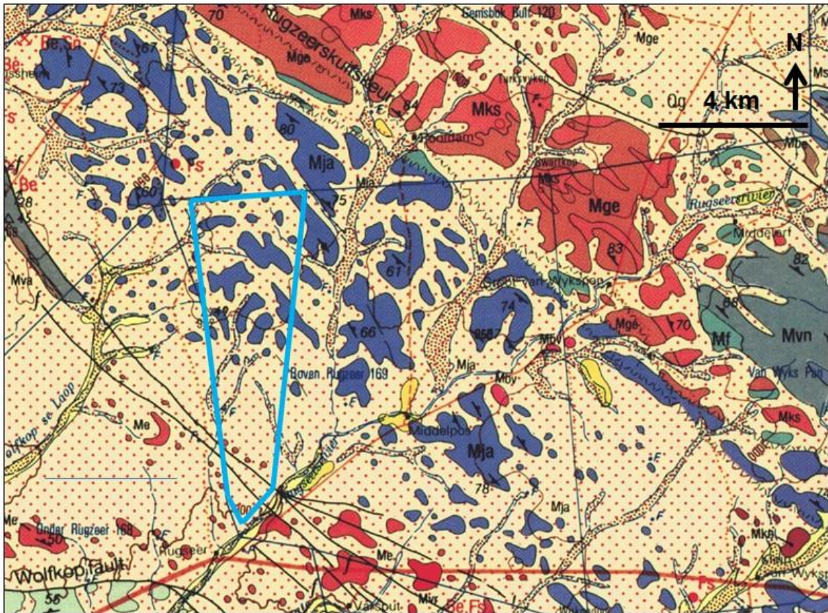
Figure 1.1. Extract from 1: 250 000 scale geological map sheet 2920 Kenhardt (Council for Geoscience, Pretoria) showing the geology of the Boven Solar PV4 study area on the Remaining Extent of Boven Rugzeer Farm 169, situated c. 30 km to the NE of Kenhardt, Northern Cape. The area – including the preferred and alternative sites as well as associated transmission lines - is approximately indicated by the pale blue polygon.
