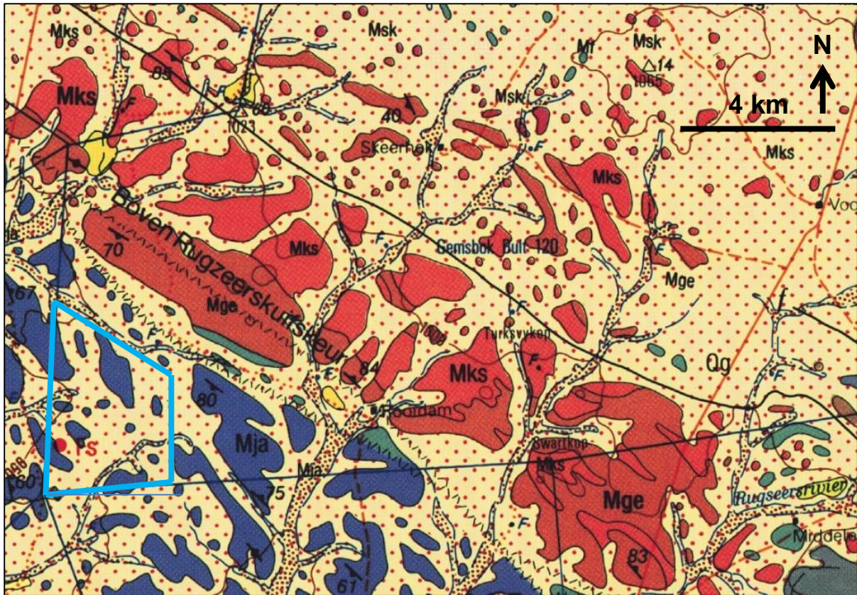
Figure 1.1. Extract from 1: 250 000 scale geological map sheet 2920 Kenhardt (Council for Geoscience, Pretoria) showing the geology of the Gembok Solar PV3 study area on the Portion 3 of Gembok Bult Farm 120, situated c. 30 km to the NE of Kenhardt, Northern Cape. The area – including the preferred and alternative sites as well as associated transmission lines - is approximately indicated by the pale blue polygon.
