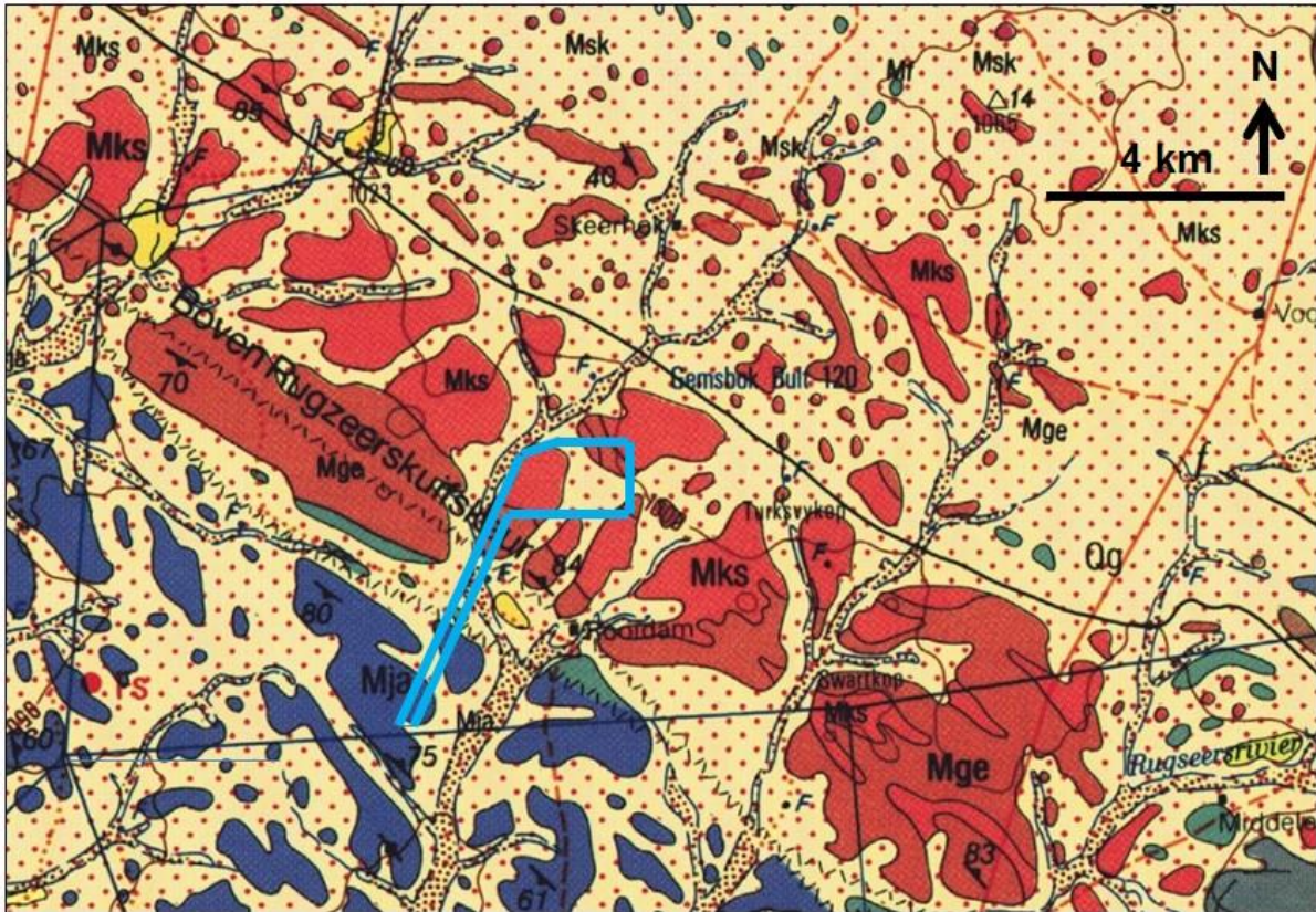
Figure 1.1. Extract from 1: 250 000 scale geological map sheet 2920 Kenhardt (Council for Geoscience, Pretoria) showing the geology of the Gembok Solar PV6 study area on the Portion 8 of Gembok Bult Farm 120, situated c. 36 km to the NE of Kenhardt, Northern Cape. The area – including the preferred and alternative sites as well as associated transmission lines - is approximately indicated by the pale blue polygon.
