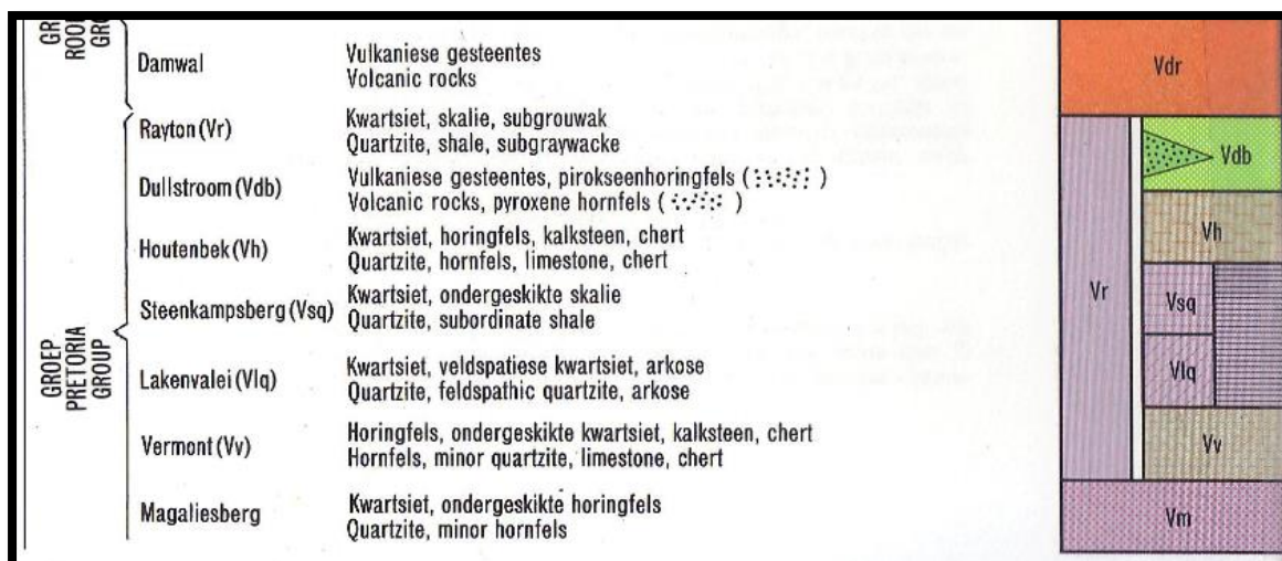
Figure 4: Lithostratigraphy (2528 Pretoria).
