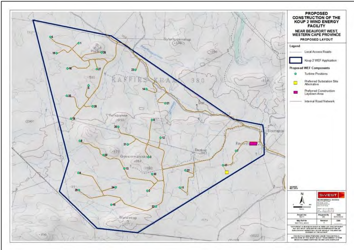
Figure 4: Proposed layout for Koup 2 WEF
