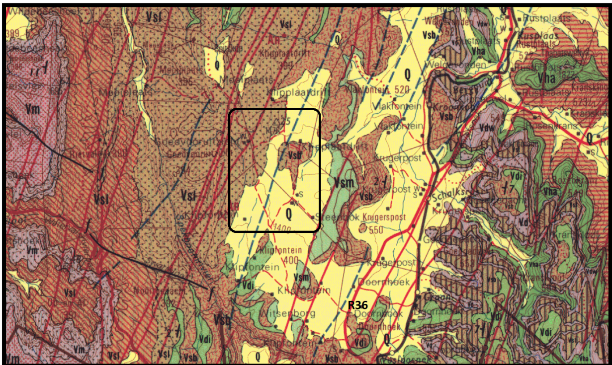
Figure 3: The geology of the development area.
