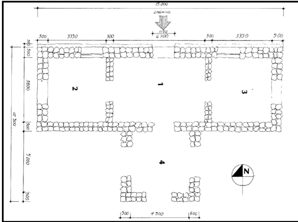
Fig. 18: Floor plan of the main house (Nienaber, 1986: 24).
