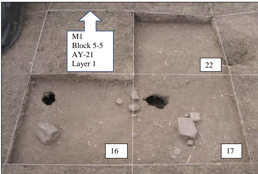
Fig. 57: The three 1x1 m blocks excavated in Midden 1.
