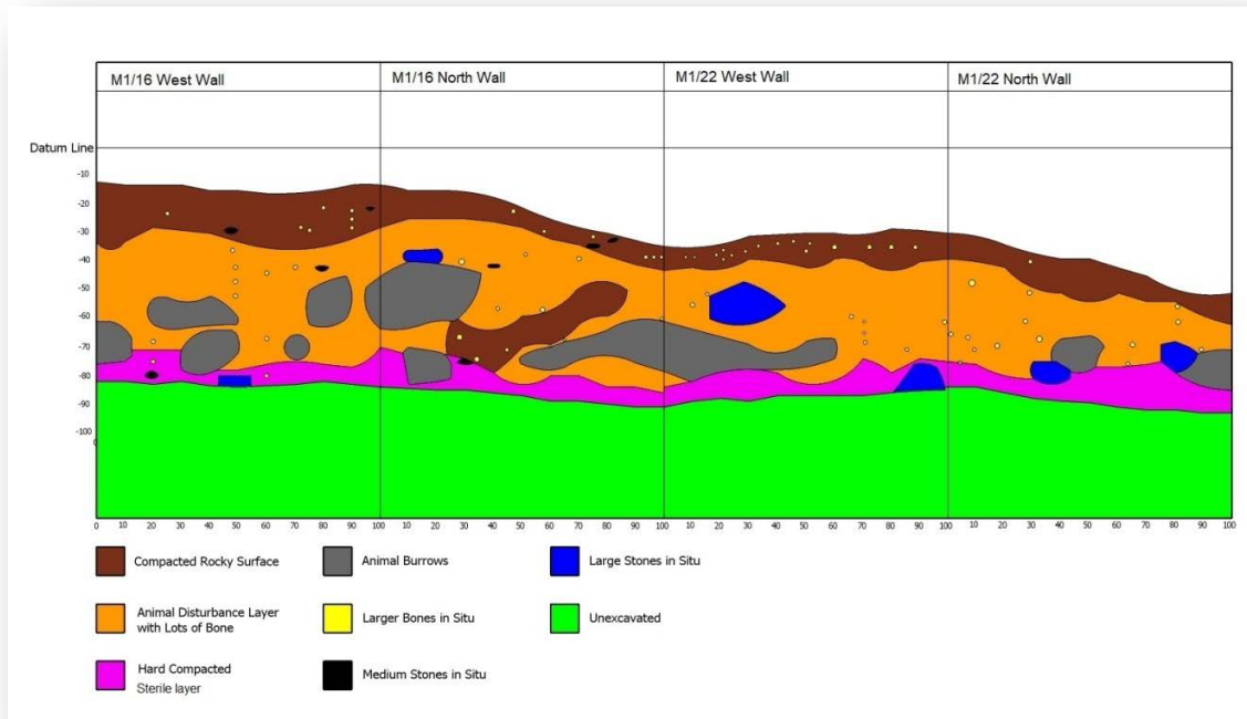
Fig. 61: The stratigraphy of blocks 16 and 22 in Midden 1.
