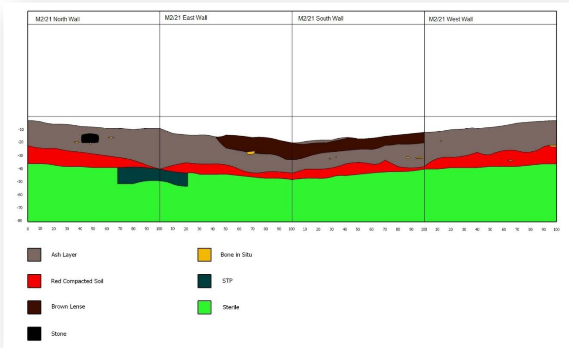
Fig. 67: Stratigraphy of block 21 in Midden 2. (Drawing; Thys Uys)
