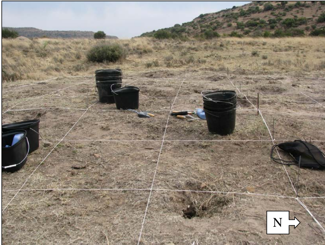
Fig. 56: The grid across Midden 1.
