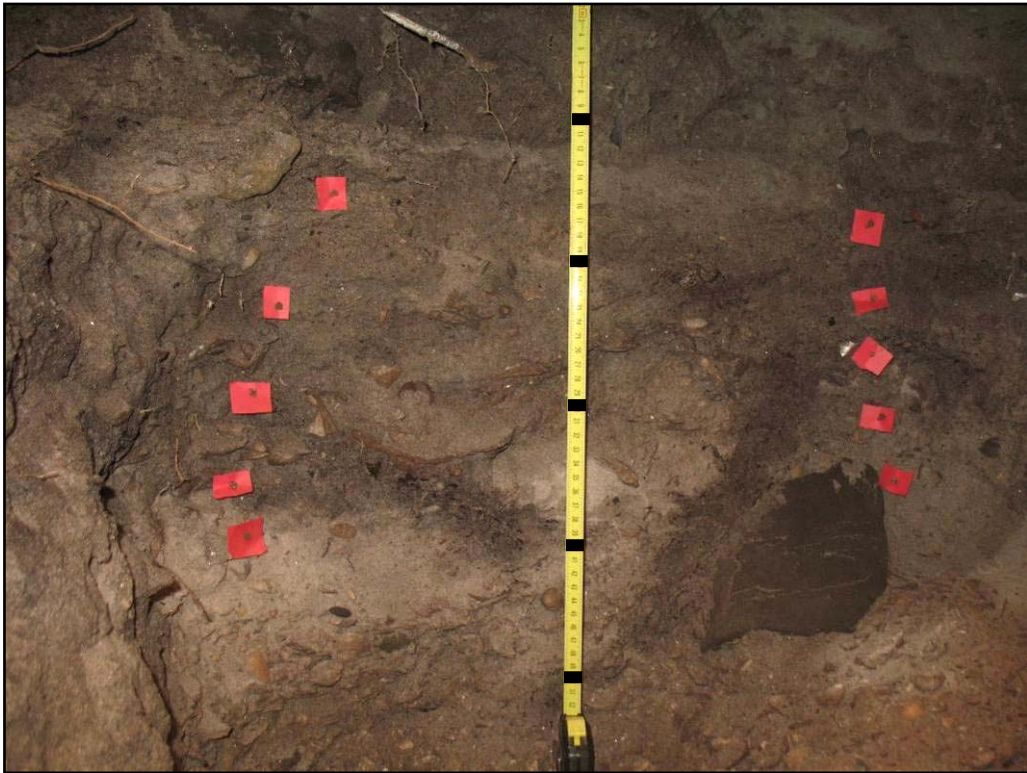
Figure 13: Close-up of the east section of J2. The black spots on the tape measure represent 10 cm intervals and the red tags indicate the base of each level (1-5). Darker disturbed soil overlies level 1.
