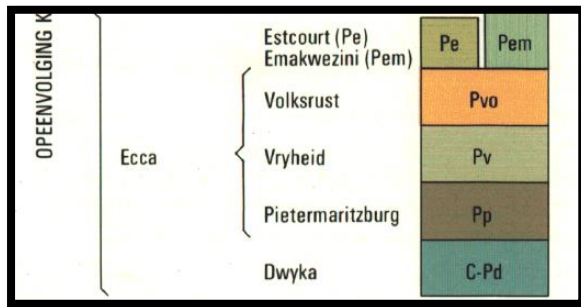
Figure 4: Lithostratigraphic column of the development area.
