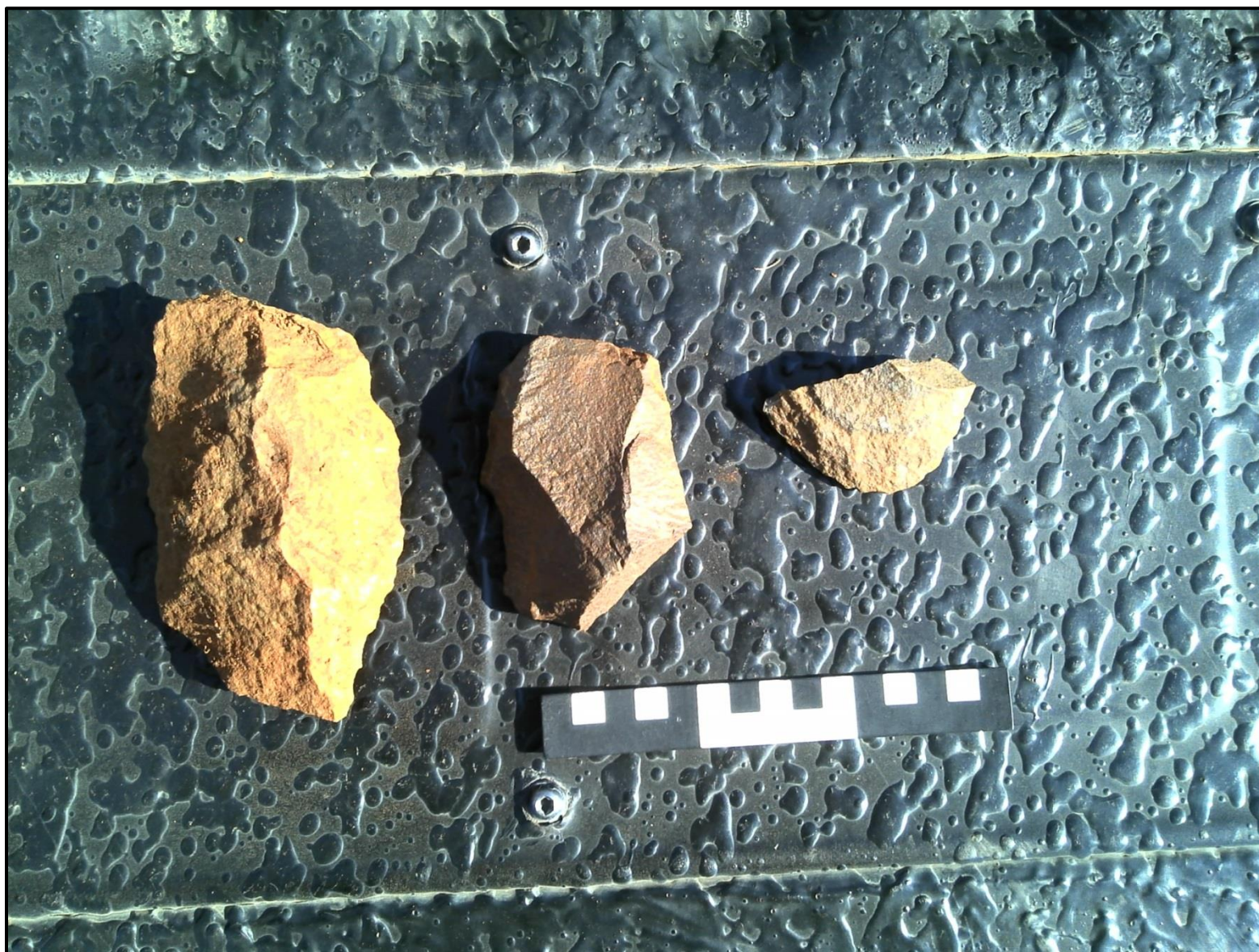
Figure 7: MSA artefacts.
