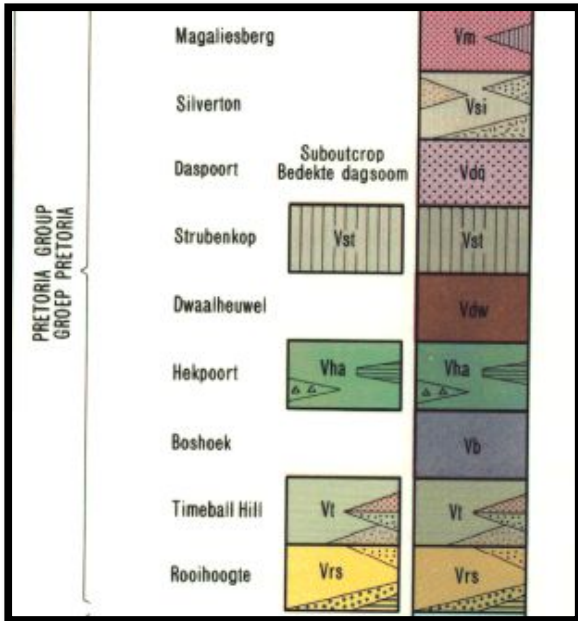
Figure 4: Lithostratigraphic column of the development area (Pretoria).
