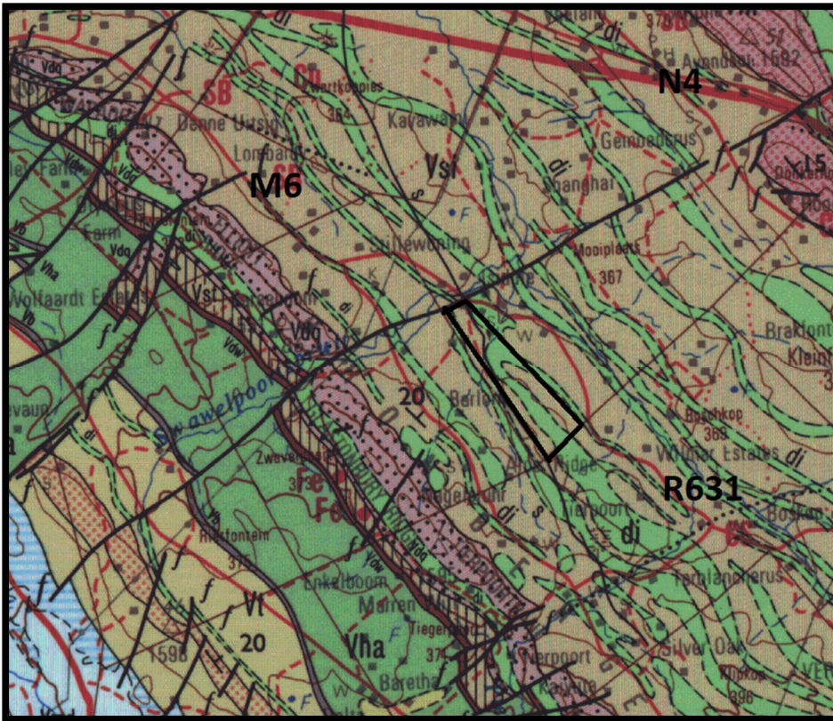
Figure 3: Geology of the development area (1h).
