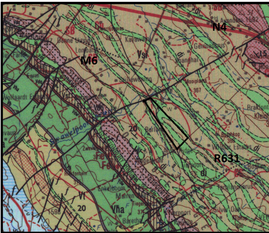
Figure: The geology of the development area.
