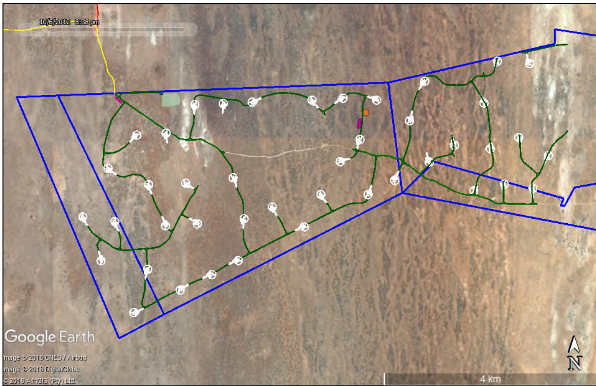
Figure 2: Aerial view of the study area showing the proposed facility layout (turbines marked in white, roads in green, substation in orange, laydown area in light green and two office buildings in pink).
