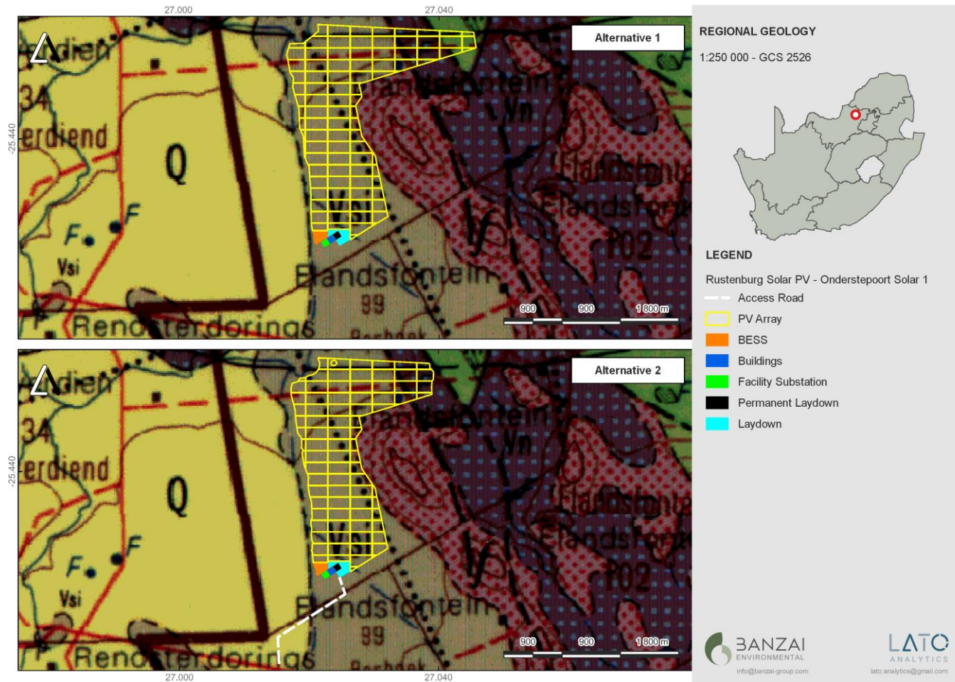
Figure 3: Extract of the 1:250 000 Rustenburg 2526 (1981) Geological Map (Council for Geosciences, Pretoria) indicating the proposed Onderstepoort Solar PV 1 Project near Rustenburg, in the North West Province. The proposed development is underlain by Quaternary aeolian sand (Q, yellow), the Silverton Formation (Vsi, khaki) as well as the Rustenburg Layered Suite.
