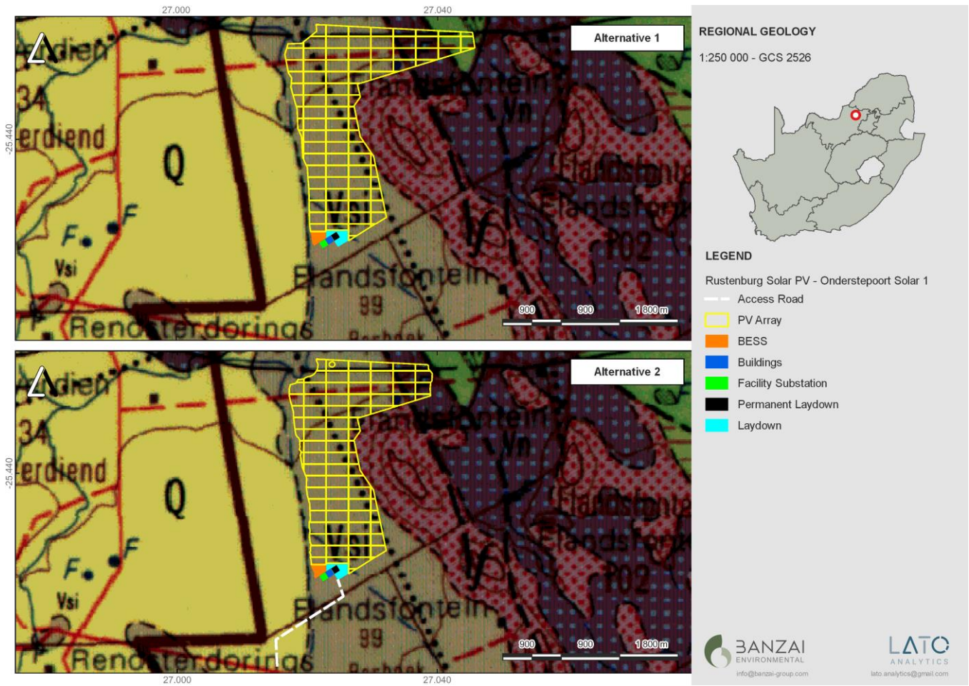
Figure S3: Extract of the 1:250 000 Rustenburg 2526 (1981) Geological Map (Council for Geosciences, Pretoria) indicating the proposed Onderstepoort Solar PV 1 Project near Rustenburg, in the North West Province. The proposed development is underlain by Quaternary aeolian sand (Q, yellow), as well as the Silverton Formation (Vsi, khaki) as well as the Rustenburg Layered Suite.
