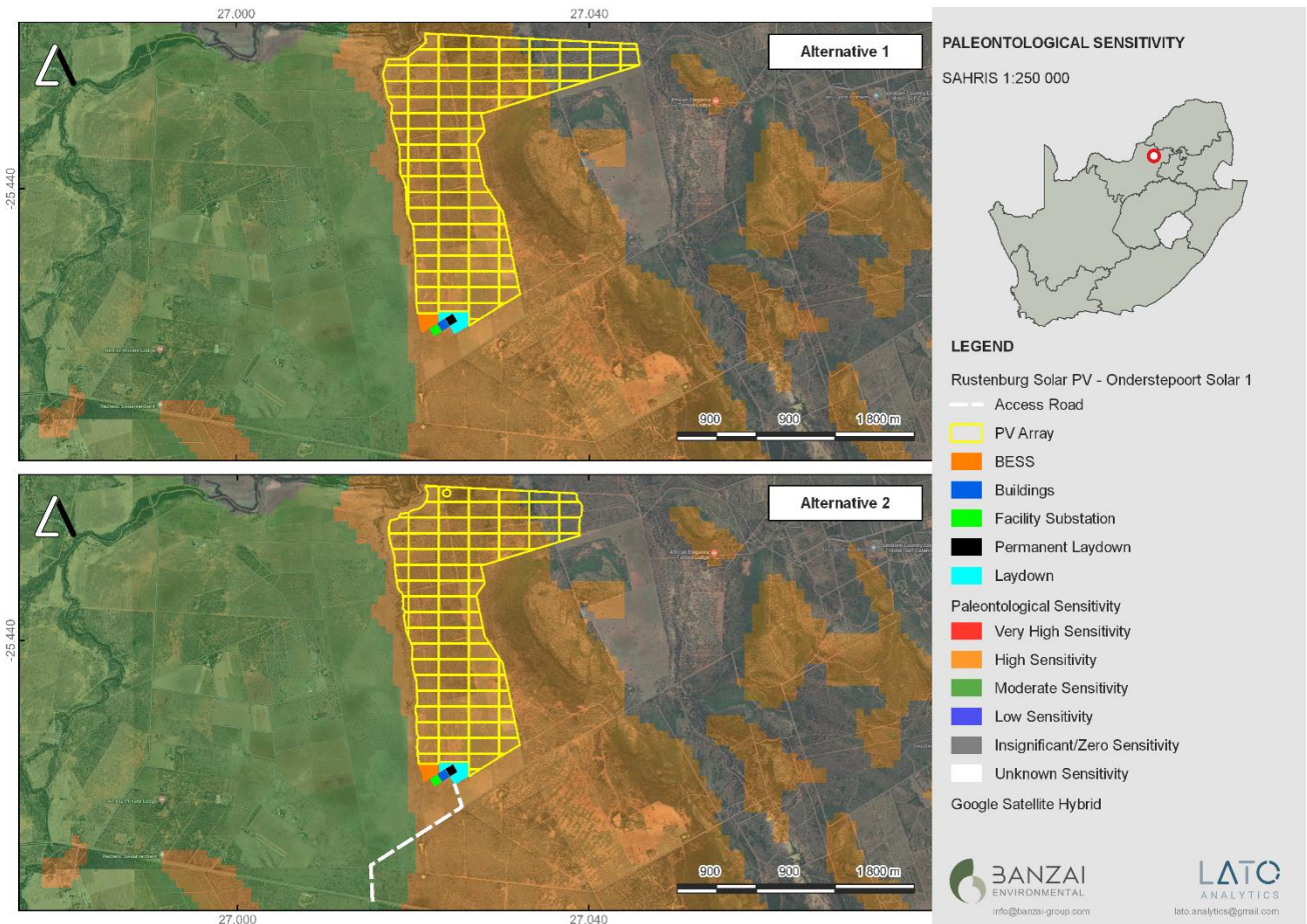
Figure 4: Extract of the 1 in 250 000 SAHRIS PalaeoMap (Council of Geosciences) indicating the proposed Onderstepoort Solar PV 1 Project near Rustenburg, in the North West Province.
