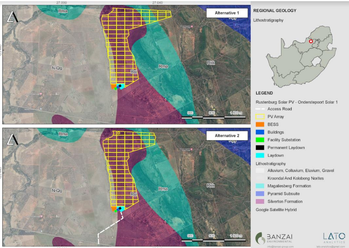
Figure 6: Updated Geology (Council of Geosciences, Pretoria) of the proposed Onderstepoort Solar PV 1 development indicates that the development is underlain by Alluvium, Elluvium, Colluvium and Gravel, as well as the Silverton and Magaliesberg Formation (Pretoria Group, Transvaal Supergroup) and the Rustenburg Layered Suite.
