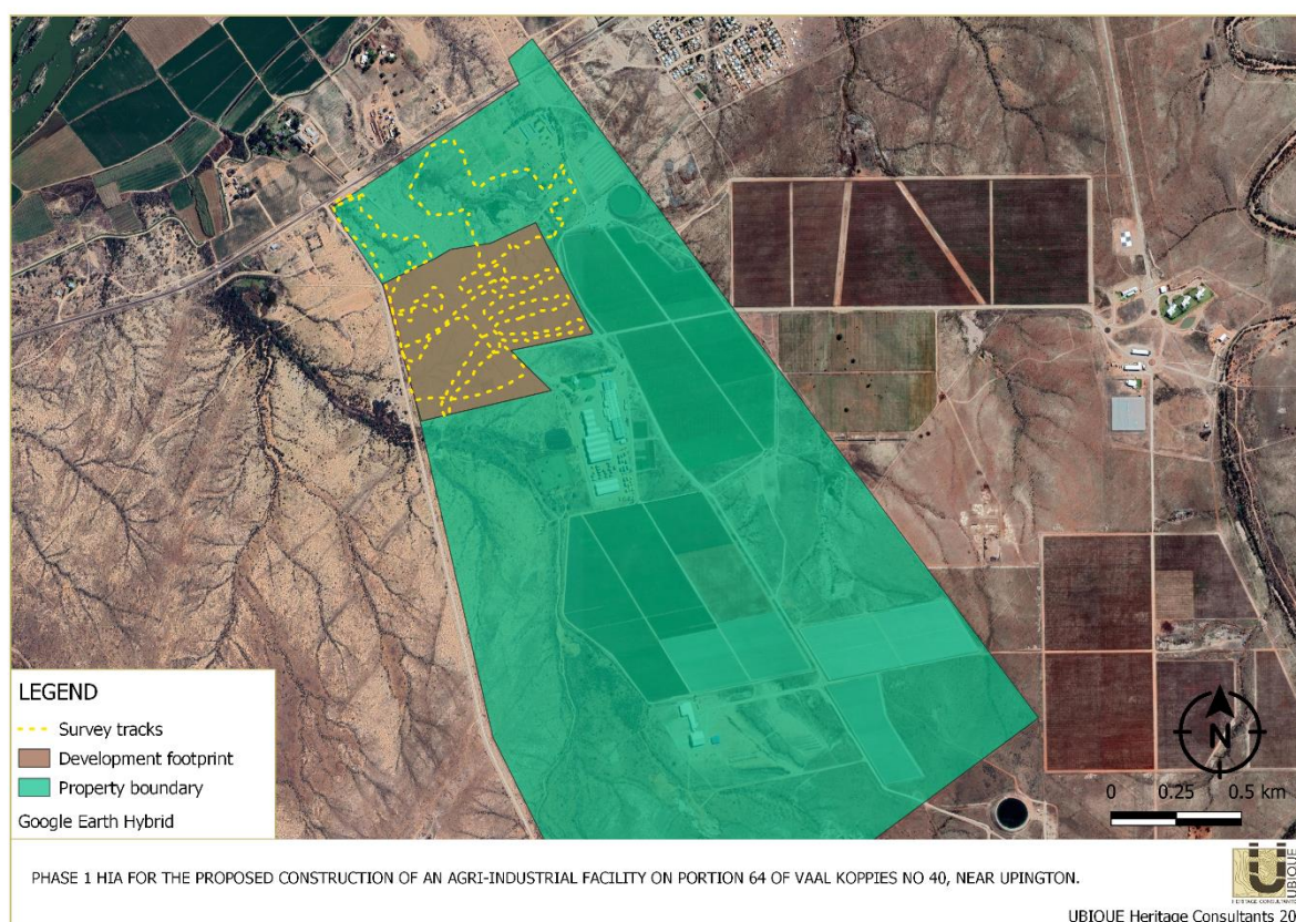
Figure 9 Survey tracks across the development footprint.
