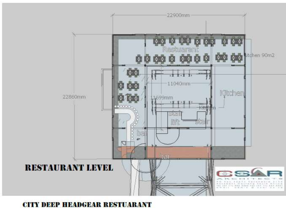
Fig.24: Drawing showing the proposed Restaurant level around the headgear (courtesy CSAR Architects).
