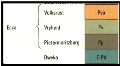
Figure 4: Lithostratigraphic column of the development area.
