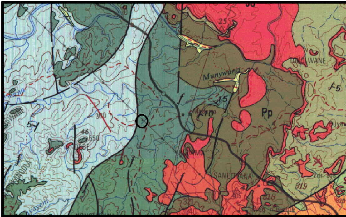
Figure 3: Geology of the development area (1h).
