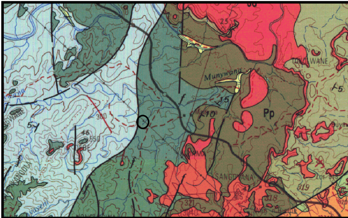
Figure: The geology of the development area (See Section F).
