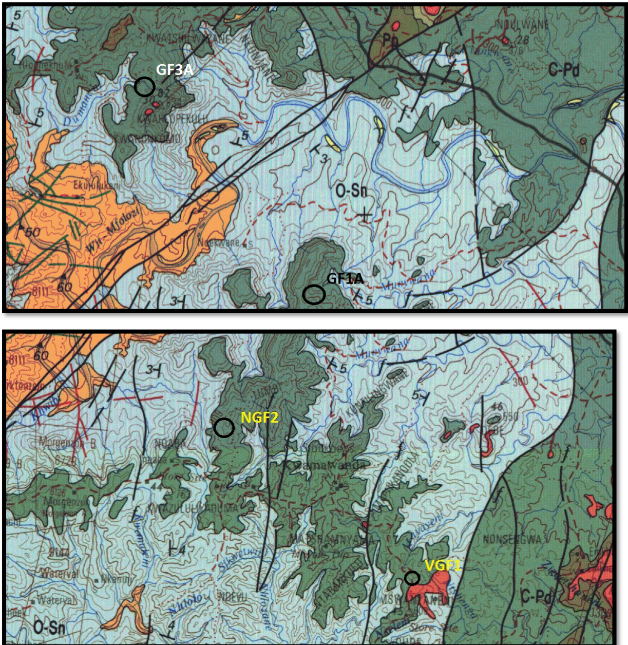
Figure 3: Geology of the development area (1h).
