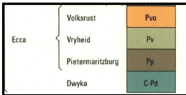
Figure 4: Lithostratigraphic column of the development area (Vryheid).
