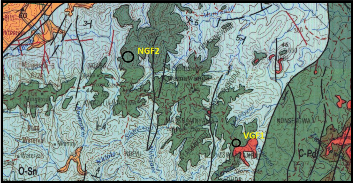
Figure: The geology of the development area (See Section F).
