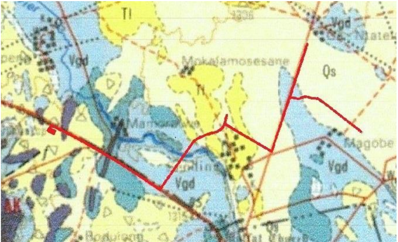
Figure 2: Geology map of the study site (red line) and surroundings. Adapted from the Kuruman 2722 1: 250 000 Geology Map (Geological Survey, 1979) and Beukes & Gutzmer (2008).
