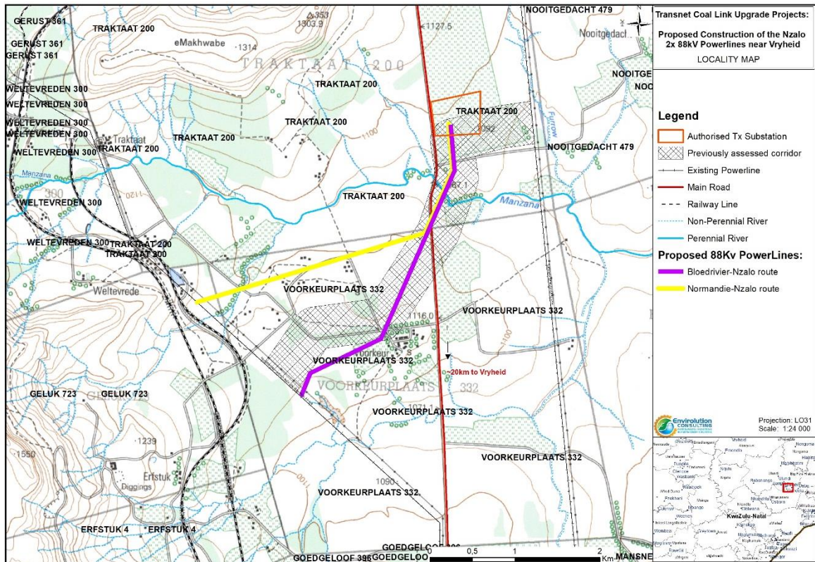
Figure 1b: Proposed Nzalo 2x 88 kV Powerlines (Envirolution).
