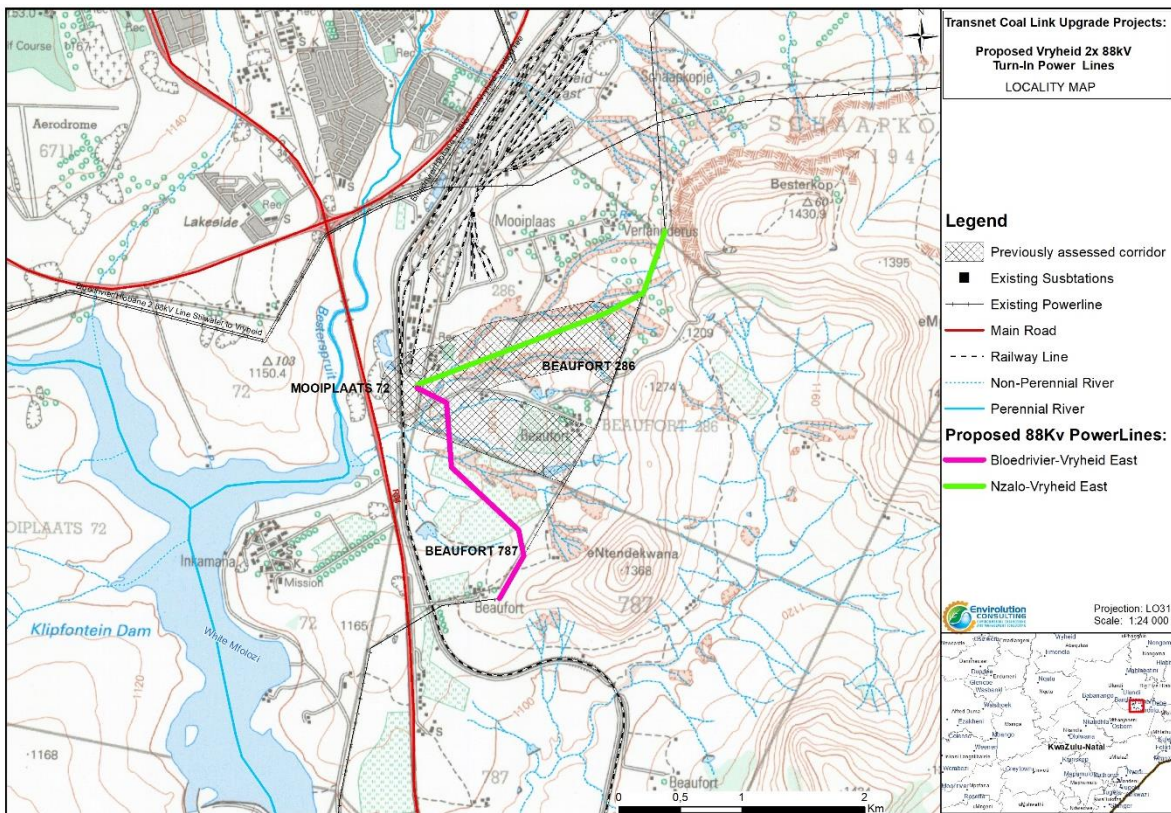
Figure 1c: Proposed Vryheid 2x 88 kV Turn-in Power Lines (Envirolution).
