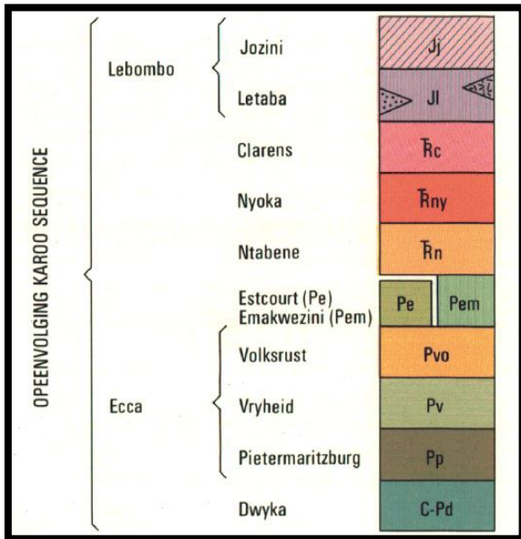
Figure 4: Lithostratigraphic column of the development area (Vryheid).
