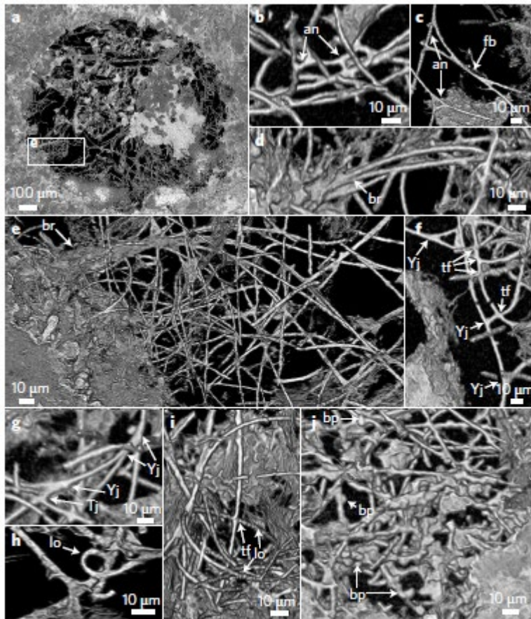
Figure 3 | Ongeluk vesicle with filamentous fossils, SRXTM surface/ volume renderings; Swedish Museum of Natural History X6137.
