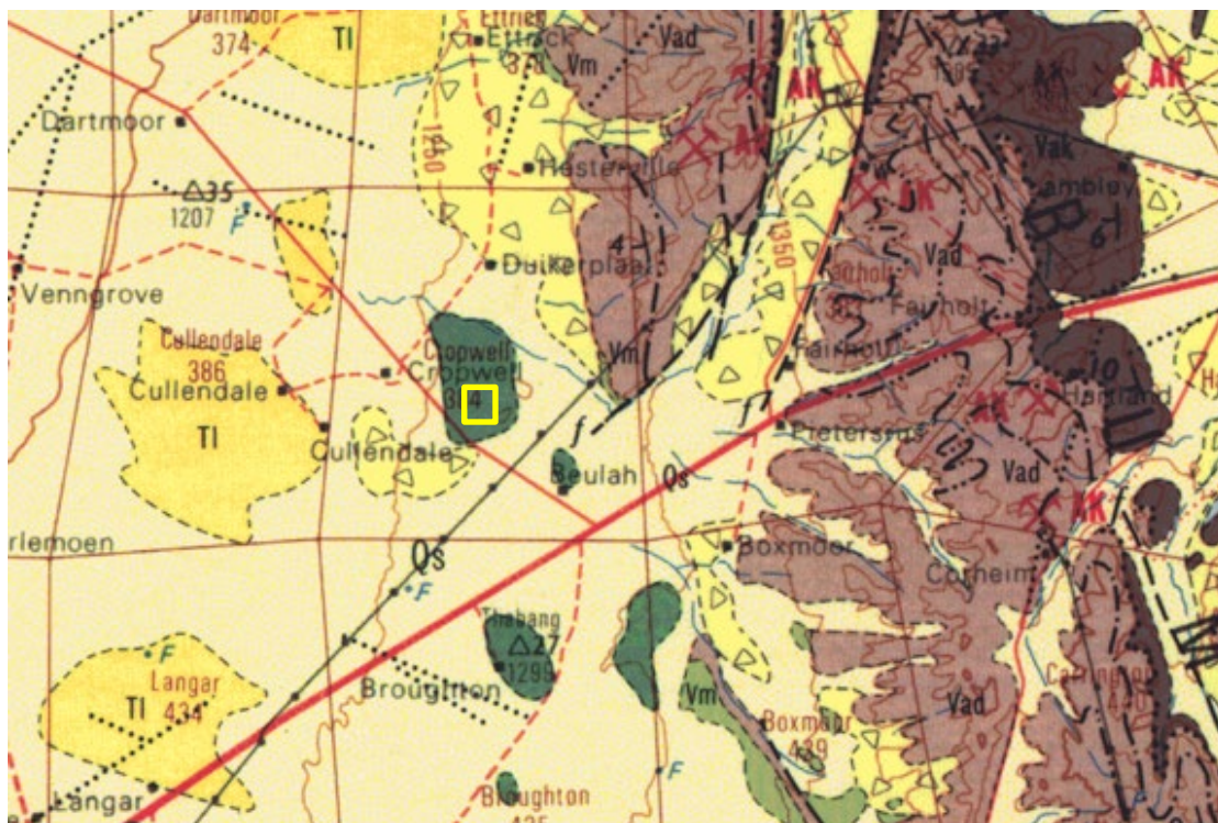
Figure 4: Geological map of the area around the Farm Cropwell 384. The location of the proposed project is indicated within the yellow rectangle. Abbreviations of the rock types are explained in Table 2. Map enlarged from the Geological Survey 1: 250 000 map 2722 Kuruman.
