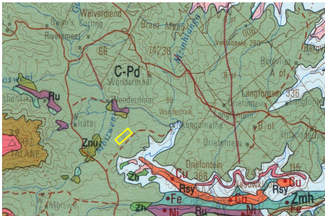
Figure 3: Geological map of the area around the Khuba Secondary School site. The location of the proposed project is indicated within the yellow rectangle. Abbreviations of the rock types are explained in Table 2. Map enlarged from the Geological Survey 1: 250 000 map 2830 Dundee.
