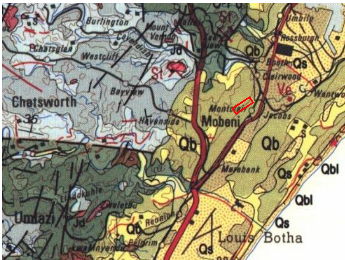
Figure 3: Geological map of the area around Mobeni and Lamontville. The location of the proposed project is indicated within the red rectangle. Abbreviations of the rock types
