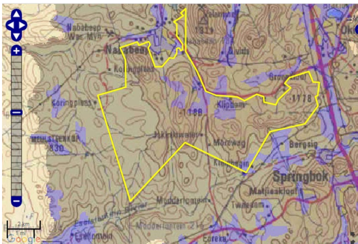
Figure 4: SAHRIS palaeosensitivity map for the site for the prospecting rights application, Farm Nababeep 134 , shown within the yellow polygon. Background colours indicate the following degrees of sensitivity: red = very highly sensitive; orange/yellow = high; green = moderate; blue = low; grey = insignificant/zero.
