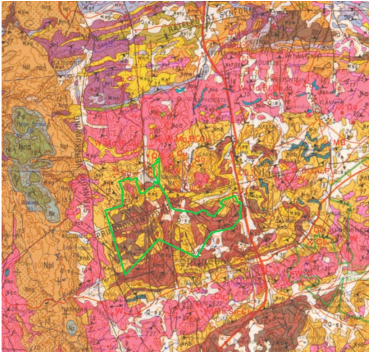
Figure 3: Geological map of the area around Nababeep. The location of the proposed project is indicated within the green polygon. Abbreviations of the rock types are explained in Table 2. Map enlarged from the Geological Survey 1: 250 000 map 2916 Springbok.
