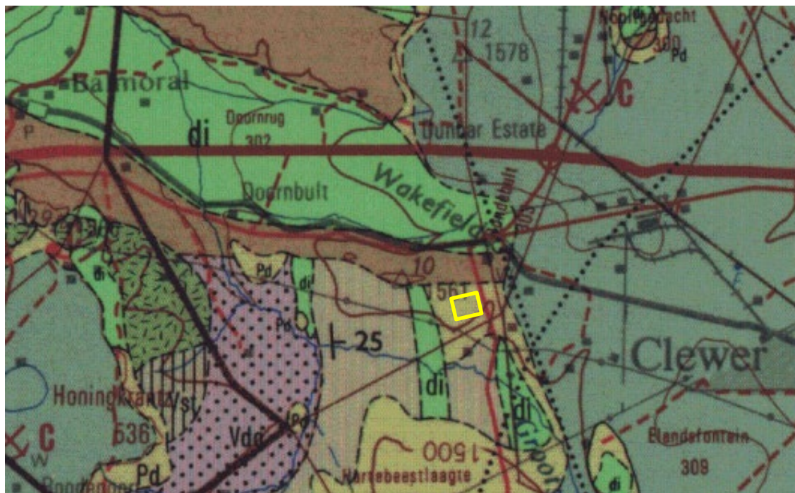
Figure 3: Geological map of the area around the proposed cemetery with the location indicated within the yellow rectangle. Abbreviations of the rock types are explained in Table 2. Map enlarged from the Geological Survey 1: 250 000 map 2528 Pretoria.
