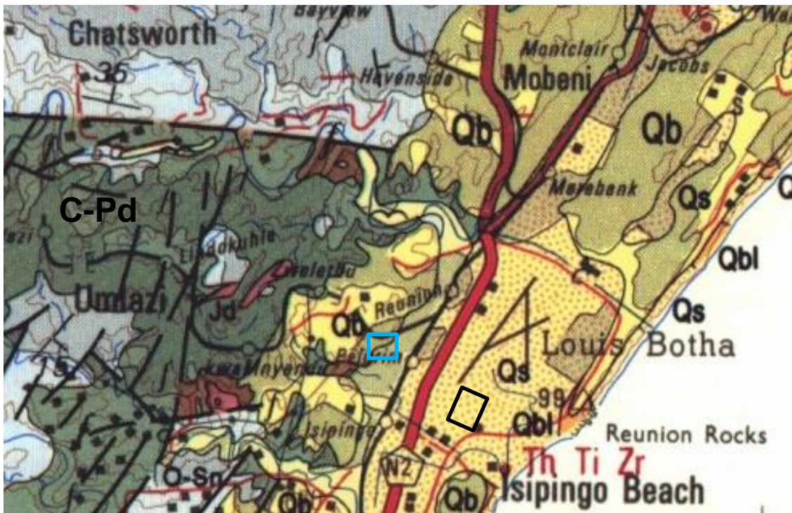
Figure 3: Geological map of the area around Pilgrim X with the site shown within the blue rectangle. Abbreviations of the rock types are explained in Table 2. Map enlarged from the Geological Survey 1: 250 000 map 2930 Durban.
