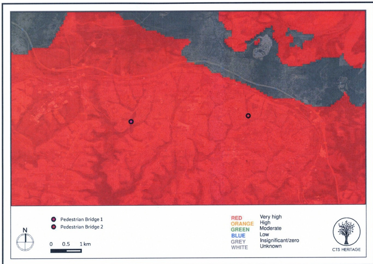
Figure 3: SAHRIS palaeosensitivity map for the site for the proposed footbridges in Mdantsane indicated by black dots. Colours indicate the following degrees of sensitivity: red = very highly sensitive; orange/yellow = high; green = moderate; blue = low; grey = insignificant/zero.
