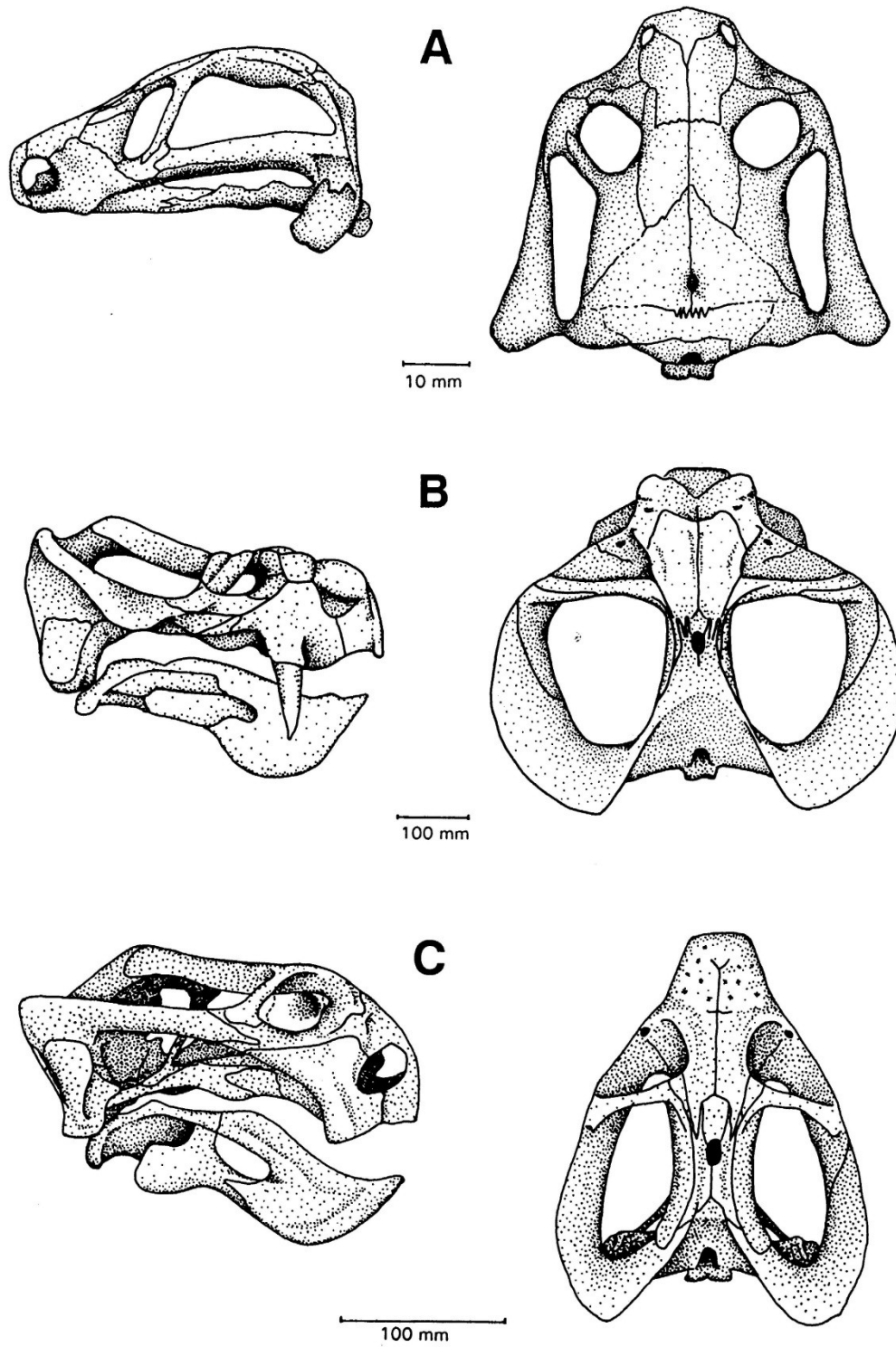
Figure 5: Cistecephalus (A), Aulacephalus (B) and Oudenodon (C) (from Rubidge et al., 1995).
