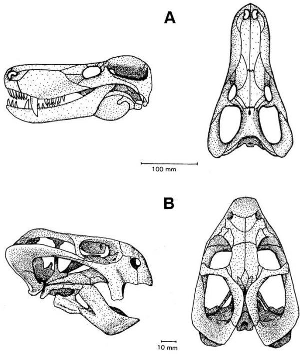
Figure 4: Pristerognathus (A) and Diictodon (B) (from Rubidge et al., 1995)
