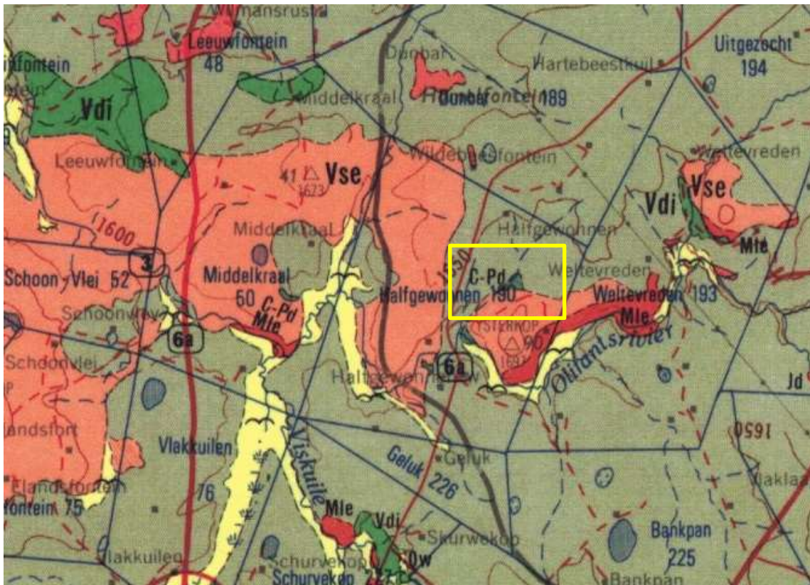
Figure 2: Geological map of the area around Halfgewonnen Farm with the proposed PV facility within the yellow outline. Abbreviations of the rock types are explained in Table 2. Map enlarged from the Geological Survey 1: 250 000 map 2628 East Rand.
