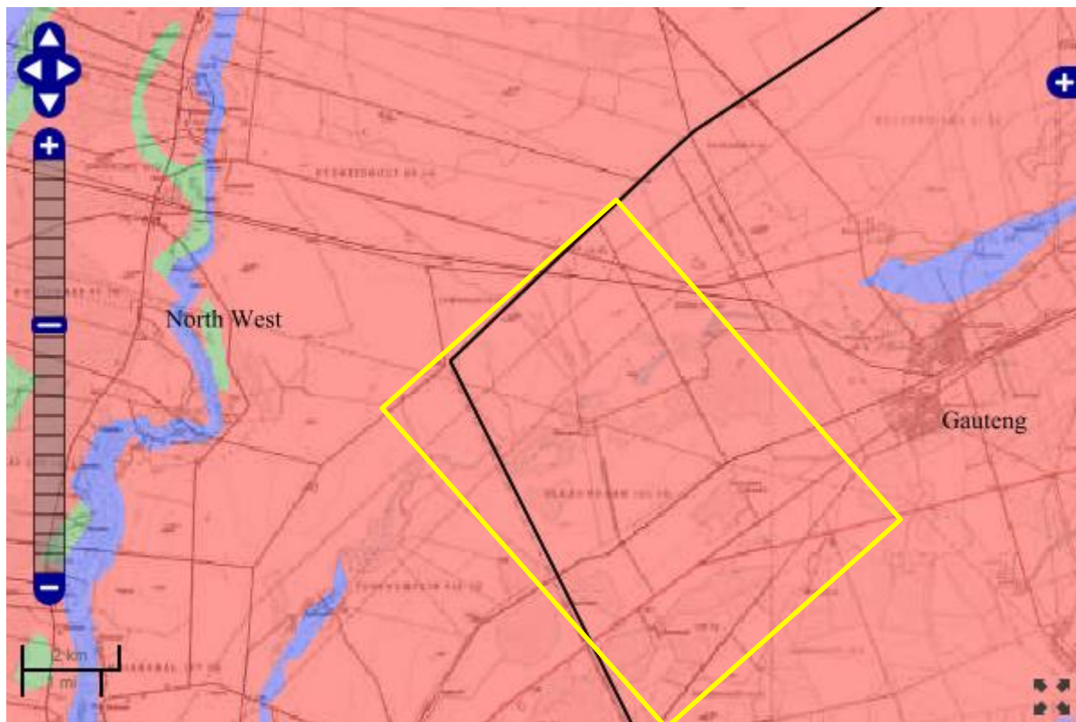
Figure 4: SAHRIS palaeosensitivity map for the site for the proposed grid connection alternates for the five Mopane PV facilities (yellow rectangle). Background colours indicate the following degrees of sensitivity: red = very highly sensitive; orange/yellow = high; green = moderate; blue = low; grey = insignificant/zero.
