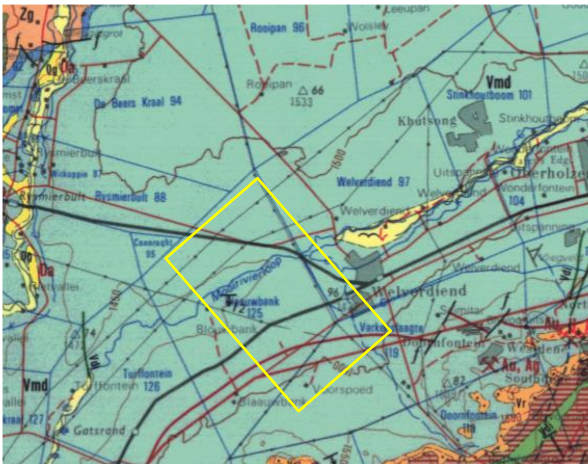
Figure 3: Geological map of the area around the proposed routes for the Mopane PVs grid
