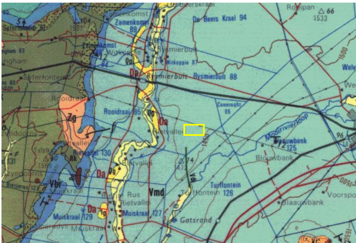
Figure 3: Geological map of the area around the Farm Rooidraai for the Mopane Solar PV 4 (yellow rectangle). Abbreviations of the rock types are explained in Table 2. Map enlarged from the Geological Survey 1: 250 000 map 2626 West Rand.
