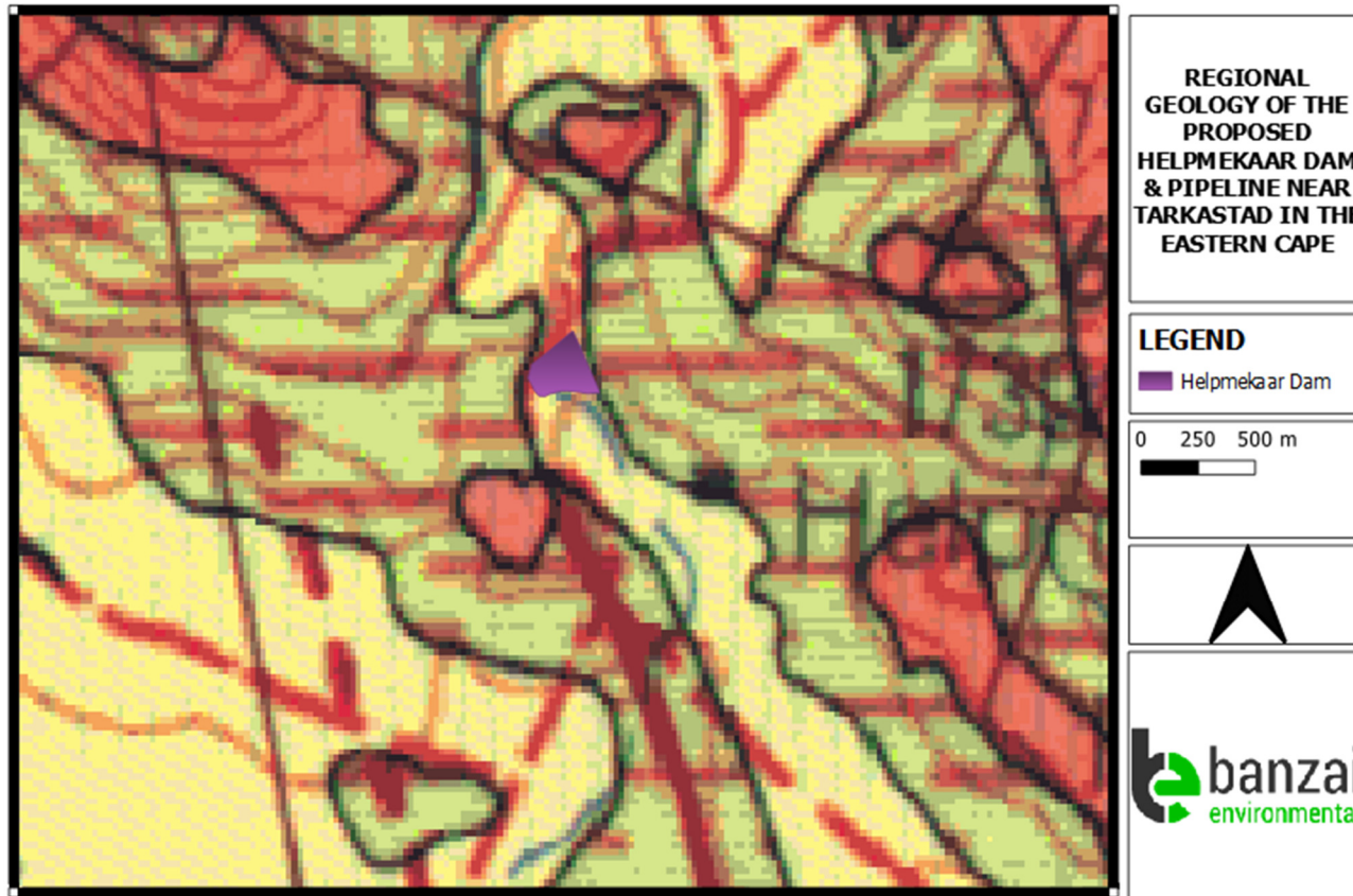
Figure 5: Extract of the 1:250 000 3126 Queenstown Geological Map (1982) (Council of Geoscience, Pretoria) indicating the locality of the proposed Helpmekaar Dam and Pipeline near Tarkastad in the Eastern Cape. Legend: Light yellow with single bird sign-Quaternary sediments; red J-D- Jurassic dolerite; Burgersdorp Formation of the Tarkastad Subgroup, Beaufort Group of the Karoo Supergroup). Map drawn by QGIS 2.18.28.
