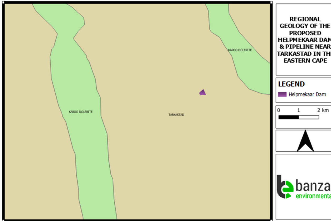
Figure 6: Shape files (Council of Geoscience, Pretoria) indicating the locality of the proposed Helpmekaar Dam and Pipeline near Tarkastad in the Eastern Cape.
