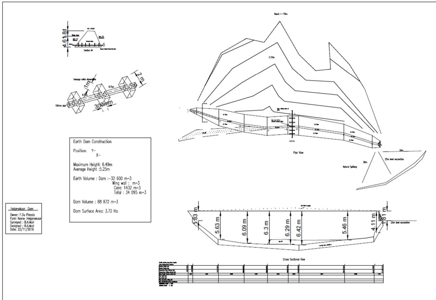
Figure 1: Proposed Helpmekaar Dam layout.
