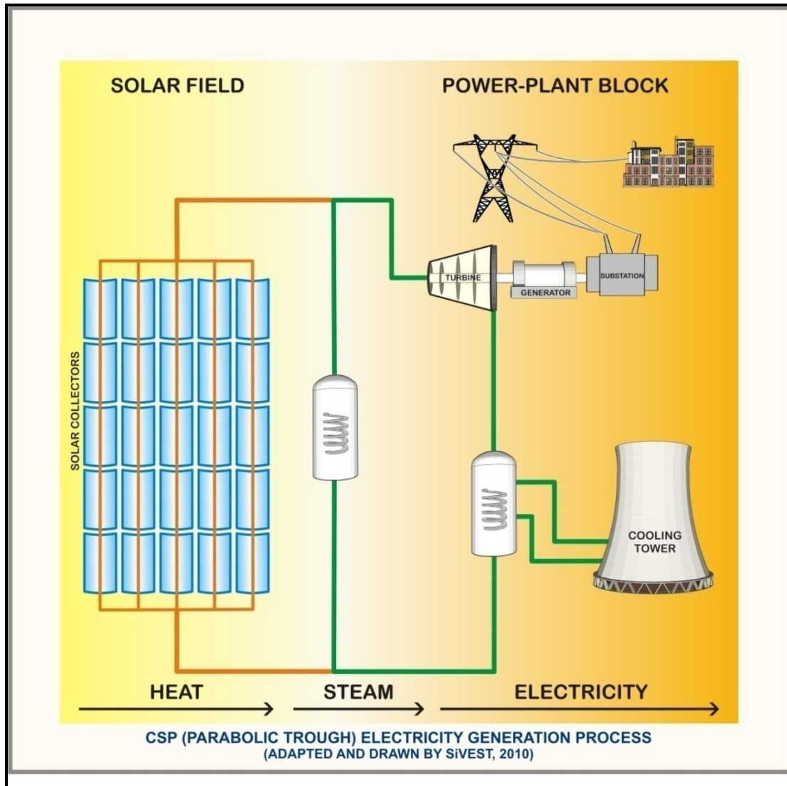
Figure 5: The CSP Process illustrated
