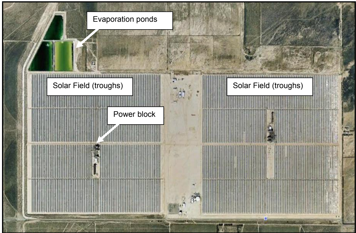
Figure 6: Google Earth Image© of the SEGS VIII and IX parabolic trough plants (Combined 160MW capacity) – Harper Lake, USA
