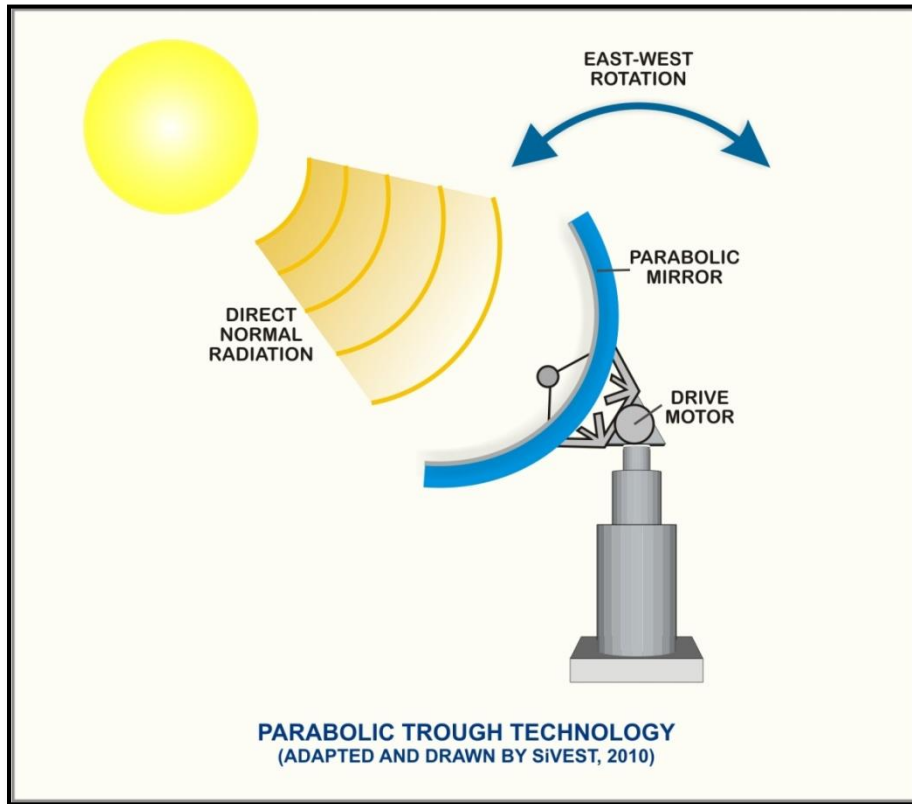
Figure 4: Functioning of the Parabolic Troughs
