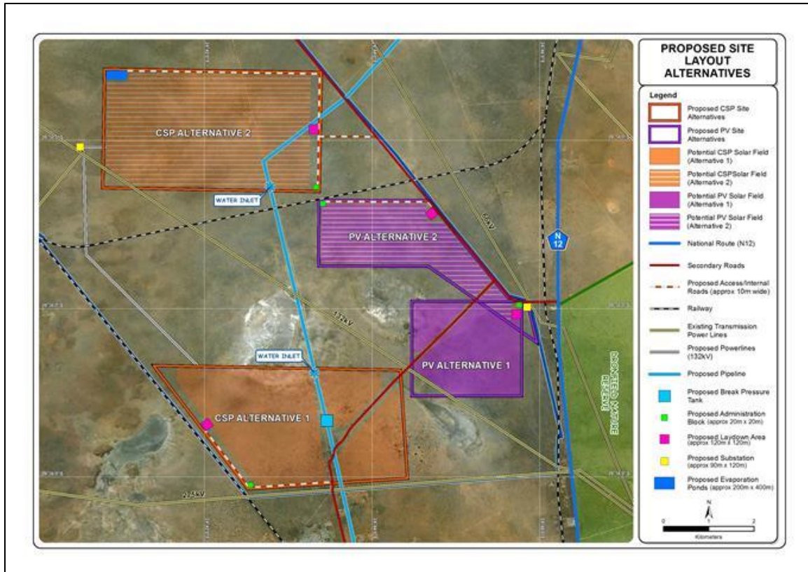
Figure 2: Droogfontein Solar Park Layout
