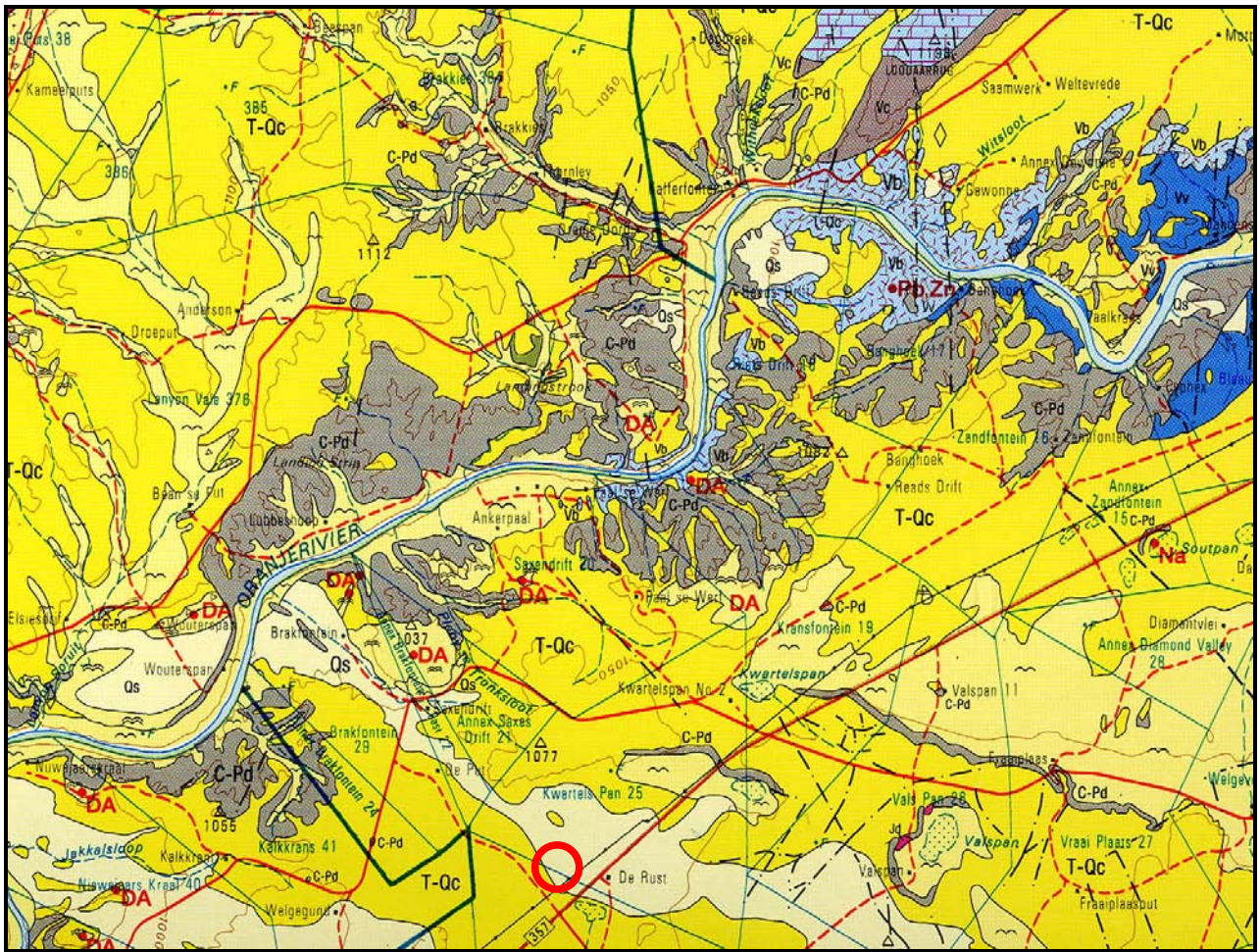
Fig. 2. Extract from 1: 250 000 geological map 2922 Prieska (Council for Geoscience, Pretoria) showing location of proposed Greefspan photovoltaic power station (red circle). Grey (C-Pd) = Dwyka Group Yellow (T-Qc) = Neogene calcrete Pale yellow (Qs) = Quaternary to Recent sands and sandy soil of the Gordonia Formation (Kalahari Group). Note mudrocks of the Prince Albert Formation (Pp) are not mapped separately in this area but might be locally present above the Dwyka Group. DA marks ancient High Level Gravels associated with alluvial diamond occurrences close to the Orange River.
