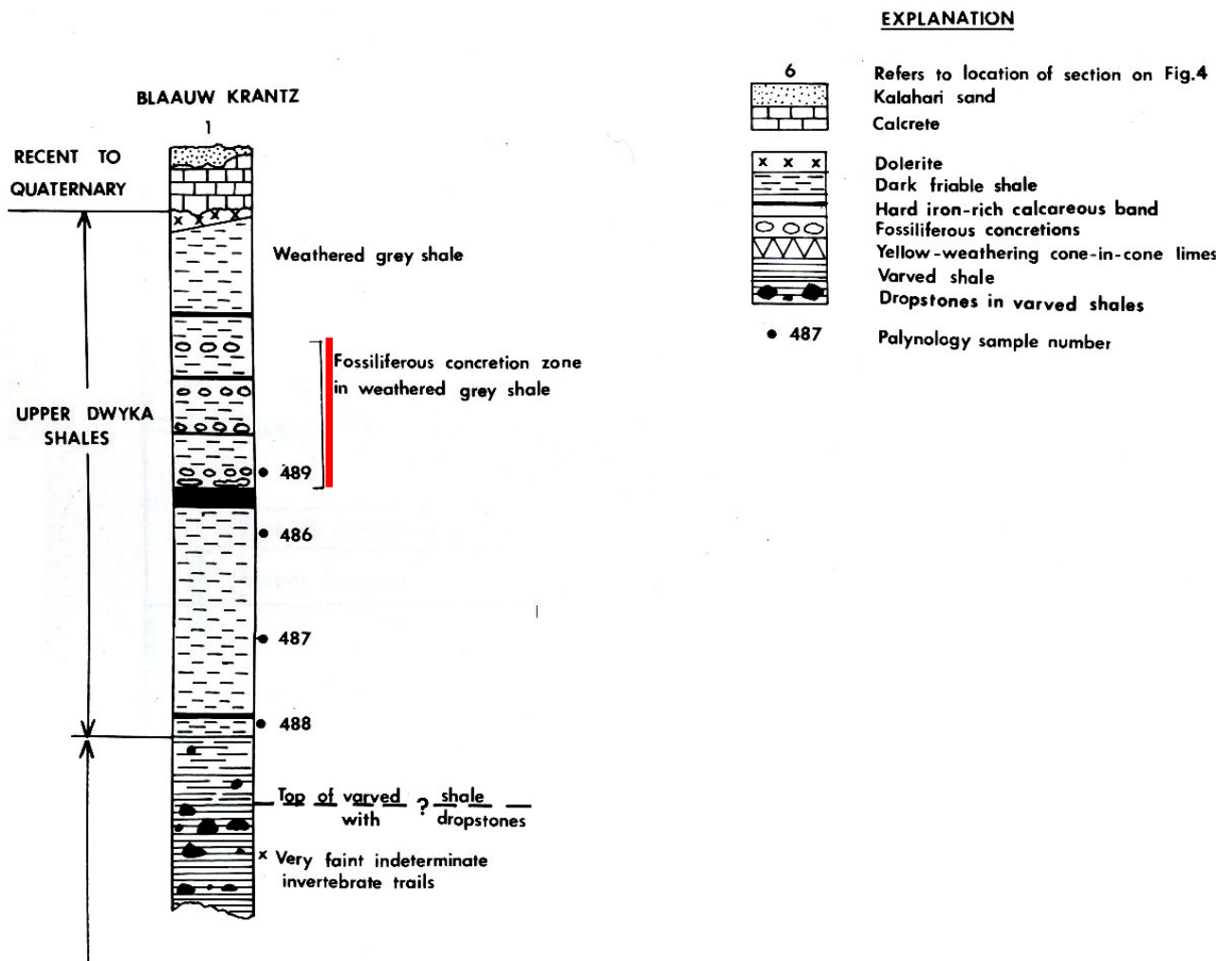
Fig. 6. Vertical section through the Dwyka / Ecca contact beds east of Douglas (See Fig. 5 above for locality area). The vertical scale is approx. 1cm = 3m. A 6m-thick zone rich in fossiliferous concretions within the Prince Albert Formation ("Upper Dwyka Shales") is emphasized by the red line. Note the Ecca beds are mantled here with a thin veneer (c. 3m) of dolerite, calcrete and Kalahari sands (= Gordonia Formation) (From McLachlan & Anderson 1973).
