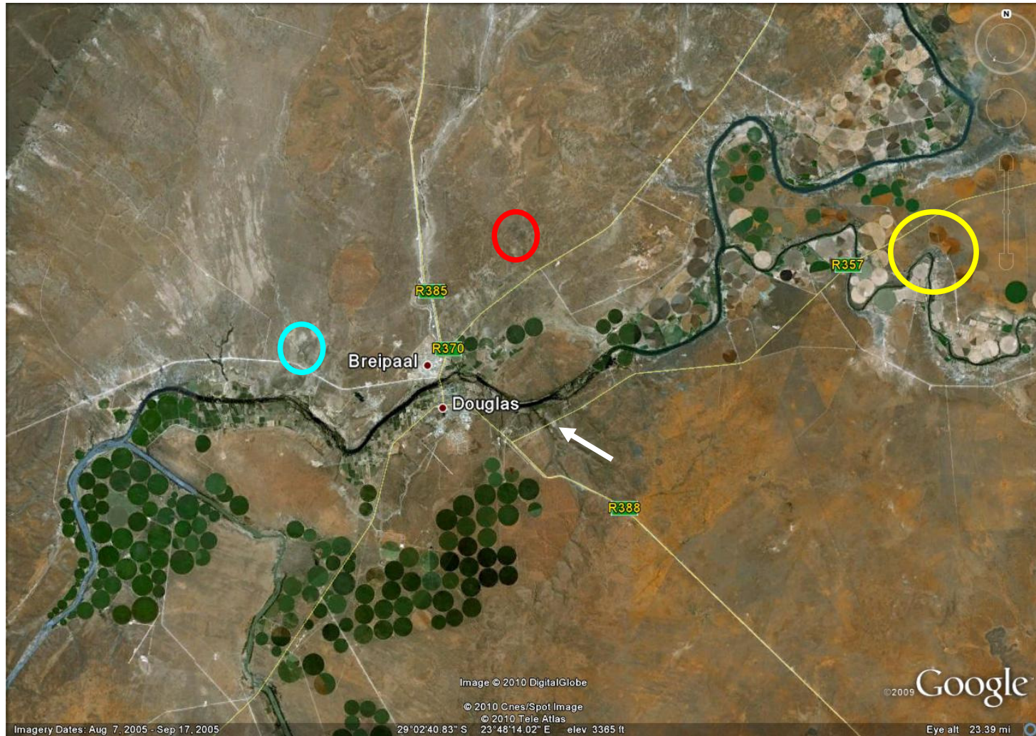
Fig. 1. Google Earth® satellite image showing the location (red circle) of the proposed photovoltaic power station at the Herbert Substation c. 7 km northeast of Douglas, Northern Cape Province. The Stratotype C section of the Mbizane Formation (Dwyka Group) on the Farm Blaauwbosdrift is indicated by the blue circle. A key fossil site within the Prince Albert Formation on the farm Blaauwkranz along the Rietrivier is indicated by the yellow circle. The white arrow indicates a borrow pit south of the R357 where the contact between calcretized High Level Gravels and the Dwyka Group is well exposed.
