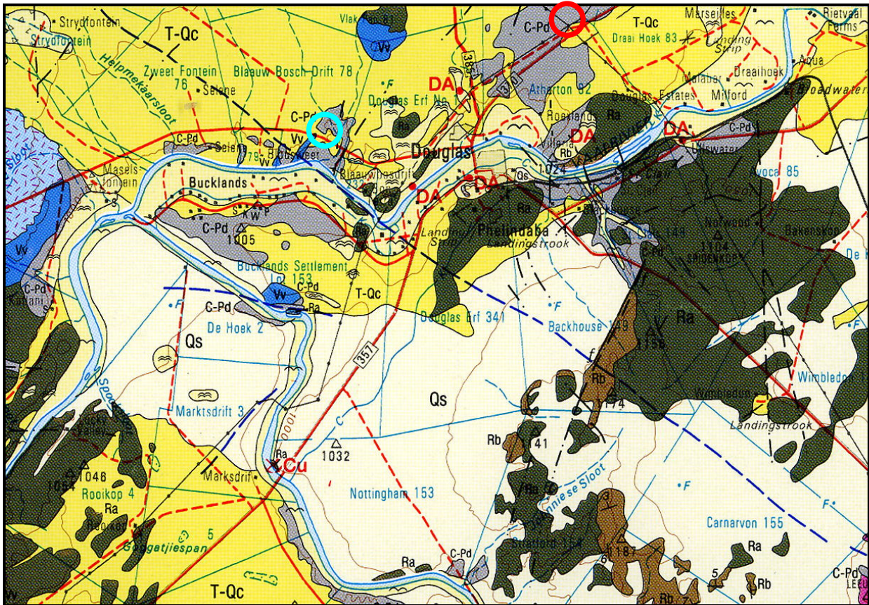
Fig. 2. Extract from 1: 250 000 geological map 2922 Prieska (Council for Geoscience, Pretoria) showing location of proposed Herbert photovoltaic power station north of the Vaal River (red circle at top edge of map). The pale blue circle to the southwest indicates the Stratotype C section of the Mbizane Formation (Dwyka Group) designated by Von Brunn & Visser (1999). This section is capped by mudrocks of Prince Albert Formation which are not separately indicated on the map.
