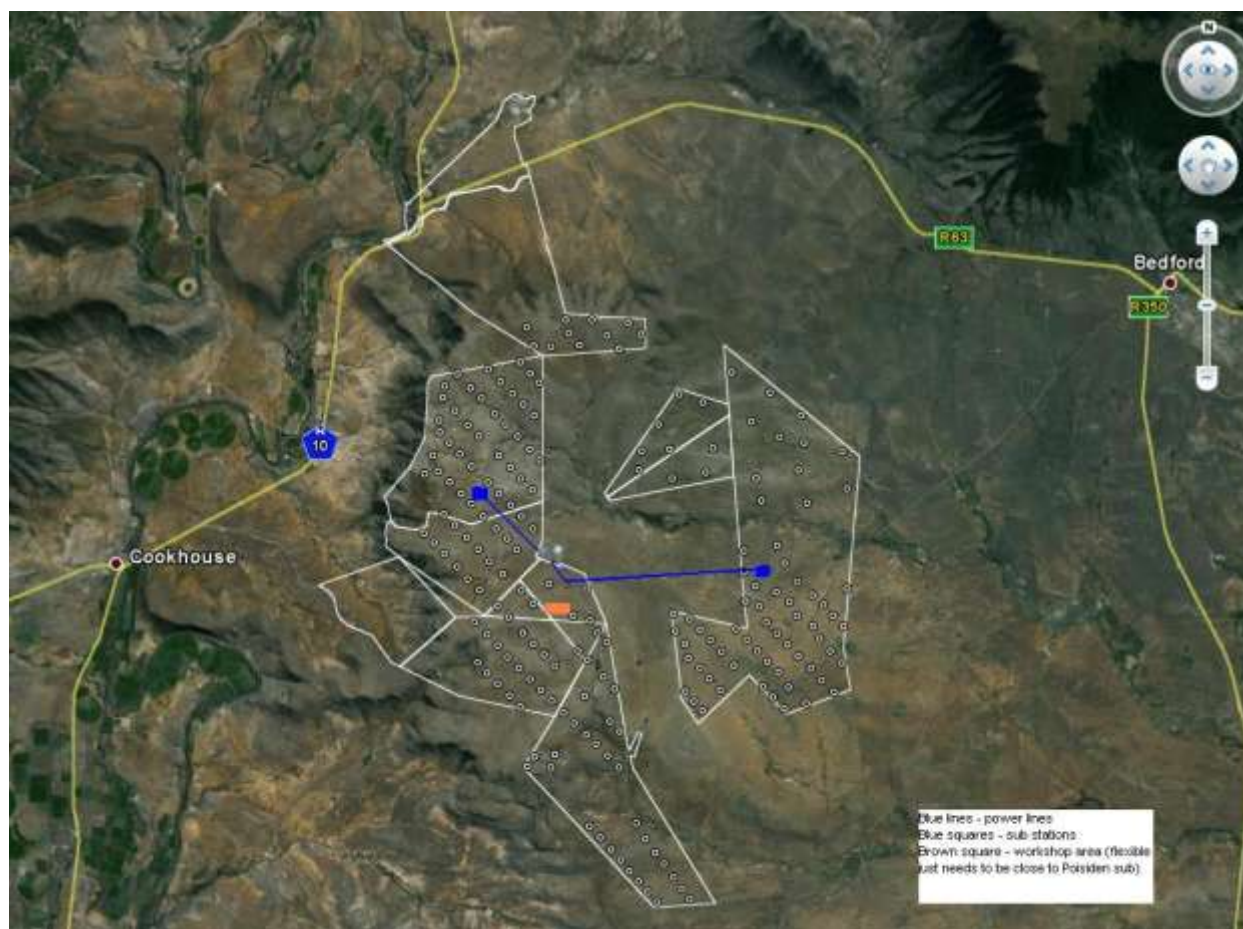
Fig. 1. Google Earth satellite image of study area spanning foothills of the Great Escarpment to the east of Cookhouse. Power lines and substations are indicated in blue. A possible location of the workshop area is shown as a brown square. See also Fig. 2 below (Image kindly provided by Savannah Environmental (Pty) Ltd).
