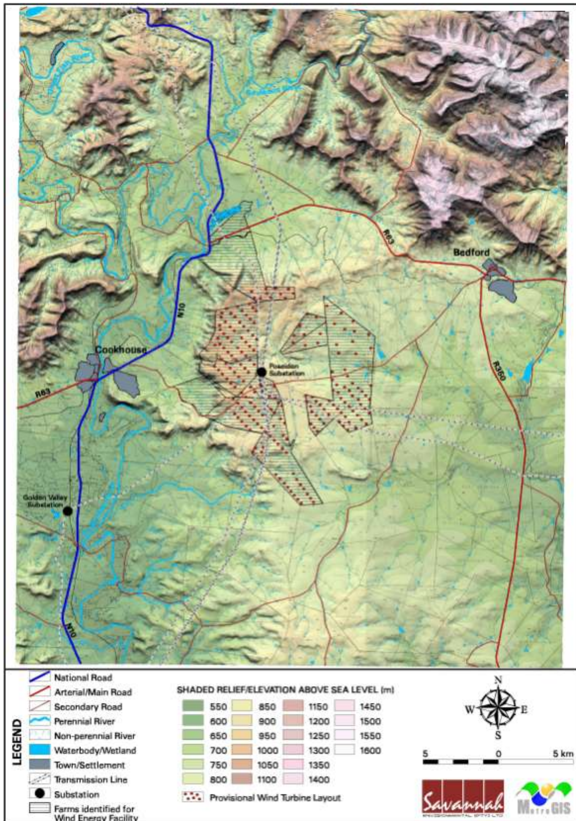
Fig. 2. Topographic map of the study area between Cookhouse and Bedford. Note the higher-lying zone towards the southern and eastern edge of the study area that is formed by prominent-weathering sandstones at the base of the Balfour Formation (Oudeberg Member). The elevated zone in the north is underlain by prominent-weathering dolerite intrusions. Compare geological map in Fig. 3 below. (Image kindly provided by Savannah Environmental (Pty) Ltd).
