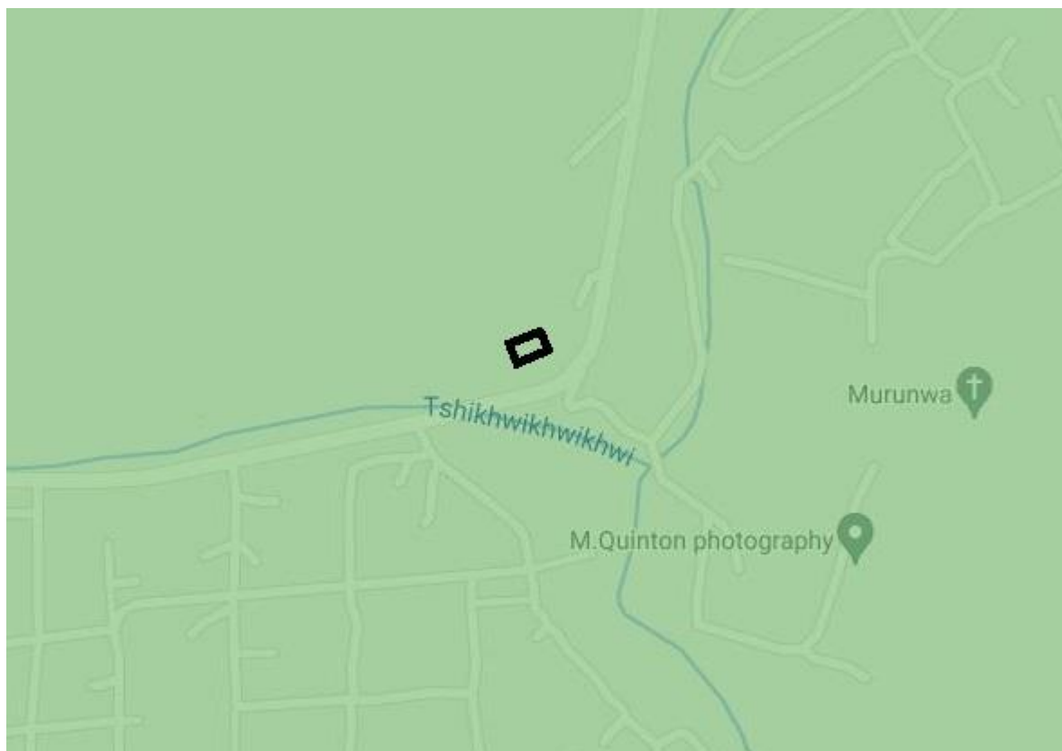
Figure 3: Palaeontological sensitivity of the study site (black polygon) (SAHRA, 2022)
