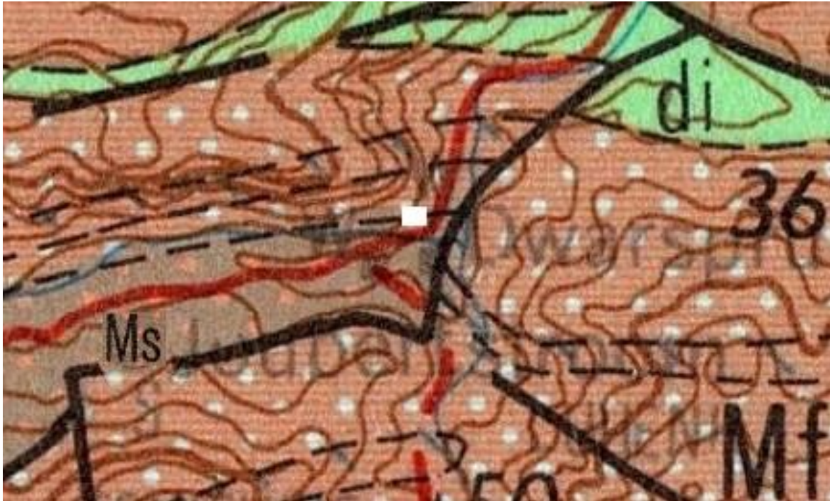
Figure 2: Geology map of the study site (white square). Adapted from the 2230 Messina 1: 250 000 Geology Map (Geological Survey, 1981)
