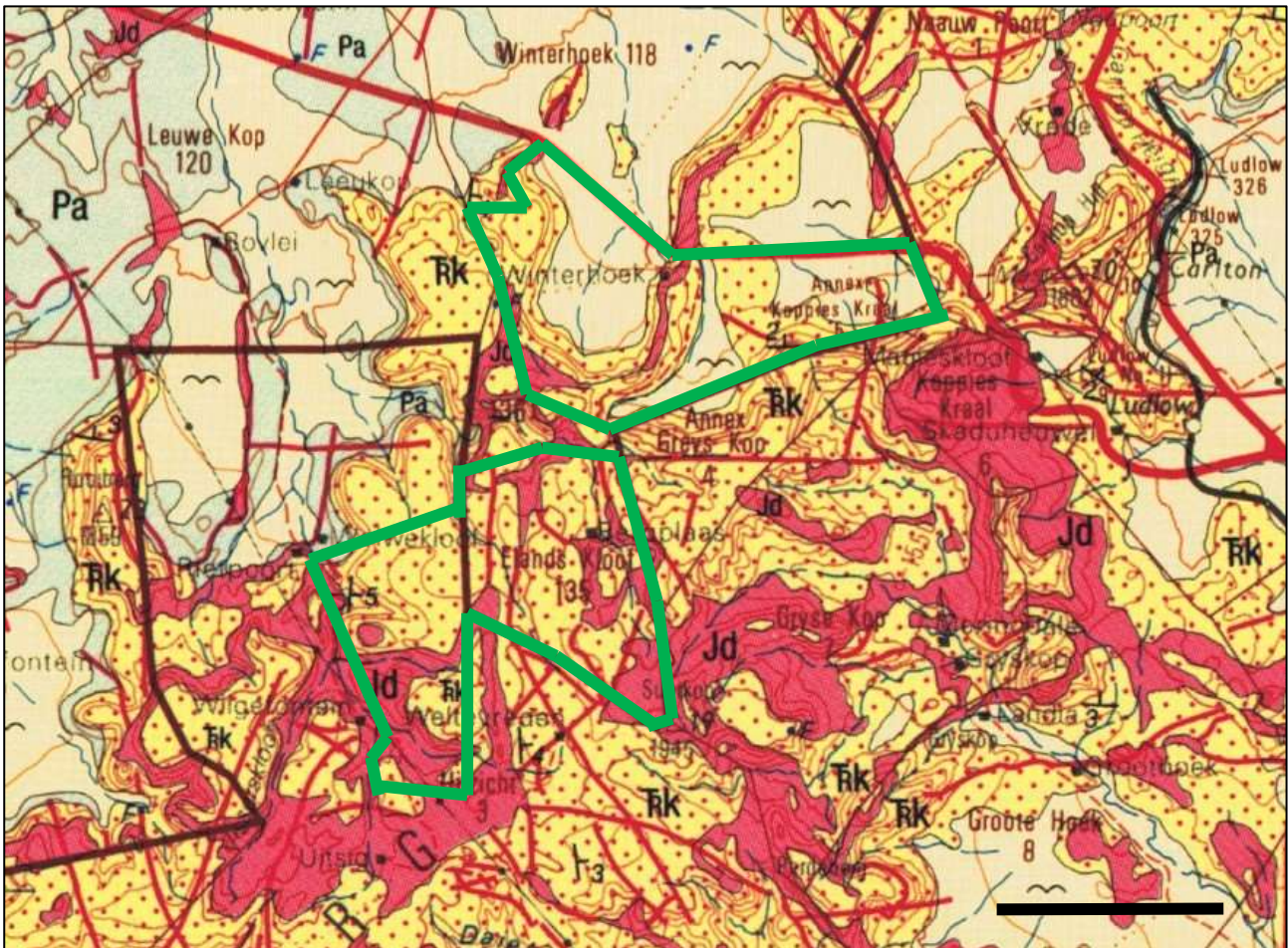
Figure 3: Extract from 1: 250 000 geology sheet 3124 Middelburg (Council for Geoscience, Pretoria) showing the approximate outline of the Umsobomvu 1 WEF and ancillary infrastructure project area in the Klein-Renosterberg region to the northwest of Middelburg, Northern and Eastern Cape (green polygon). Scale bar = 4 km. N towards the top of the map. The main geological units represented here are: Pa (pale blue-green) = Late Permian to Earliest Triassic Adelaide Subgroup (Lower Beaufort Group, Karoo Supergroup); TRk (pale orange with red dots) = Early Triassic Katberg Formation of the Tarkastad Subgroup (Upper Beaufort Group, Karoo Supergroup); Jd (red) = intrusive sills and dykes of the Early
