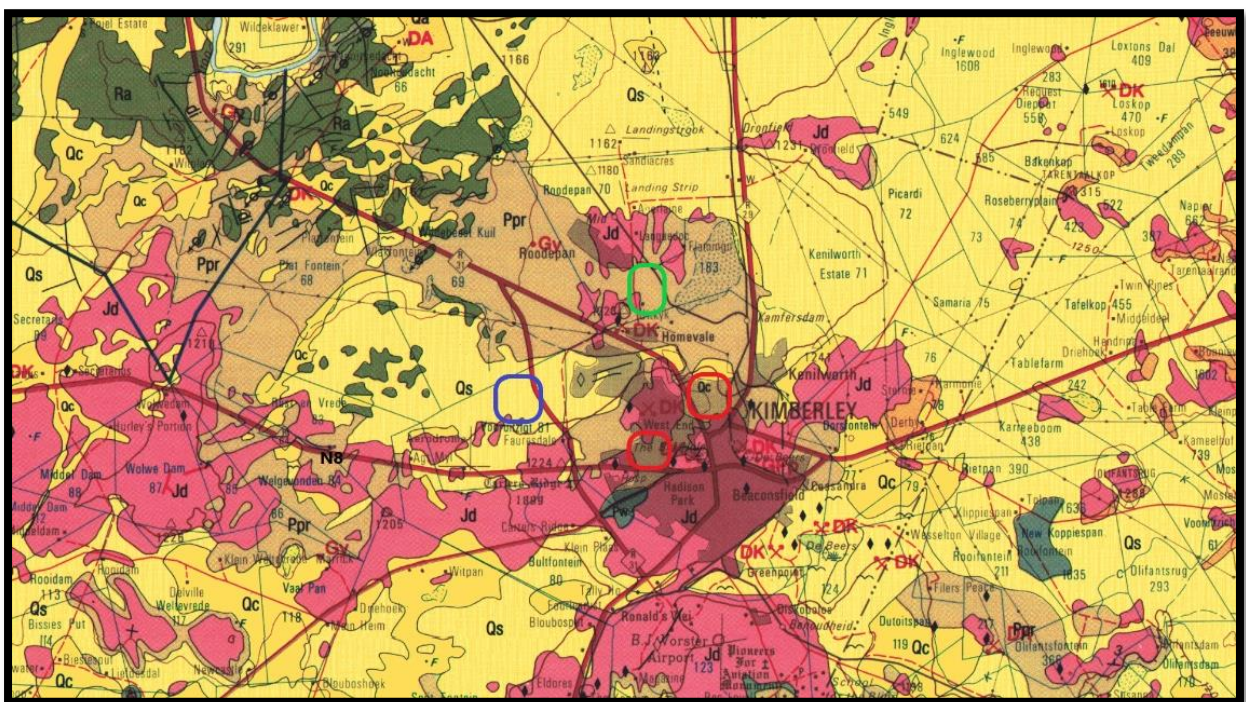
Figure 3: The geology of the development area.
