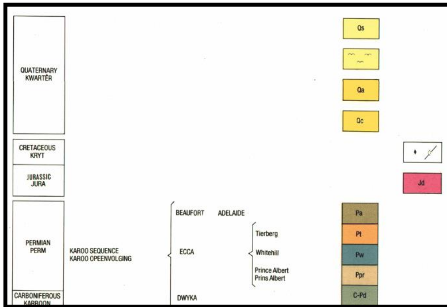
Figure 4: Lithostratigraphy (Bosch and Visser 1994).
