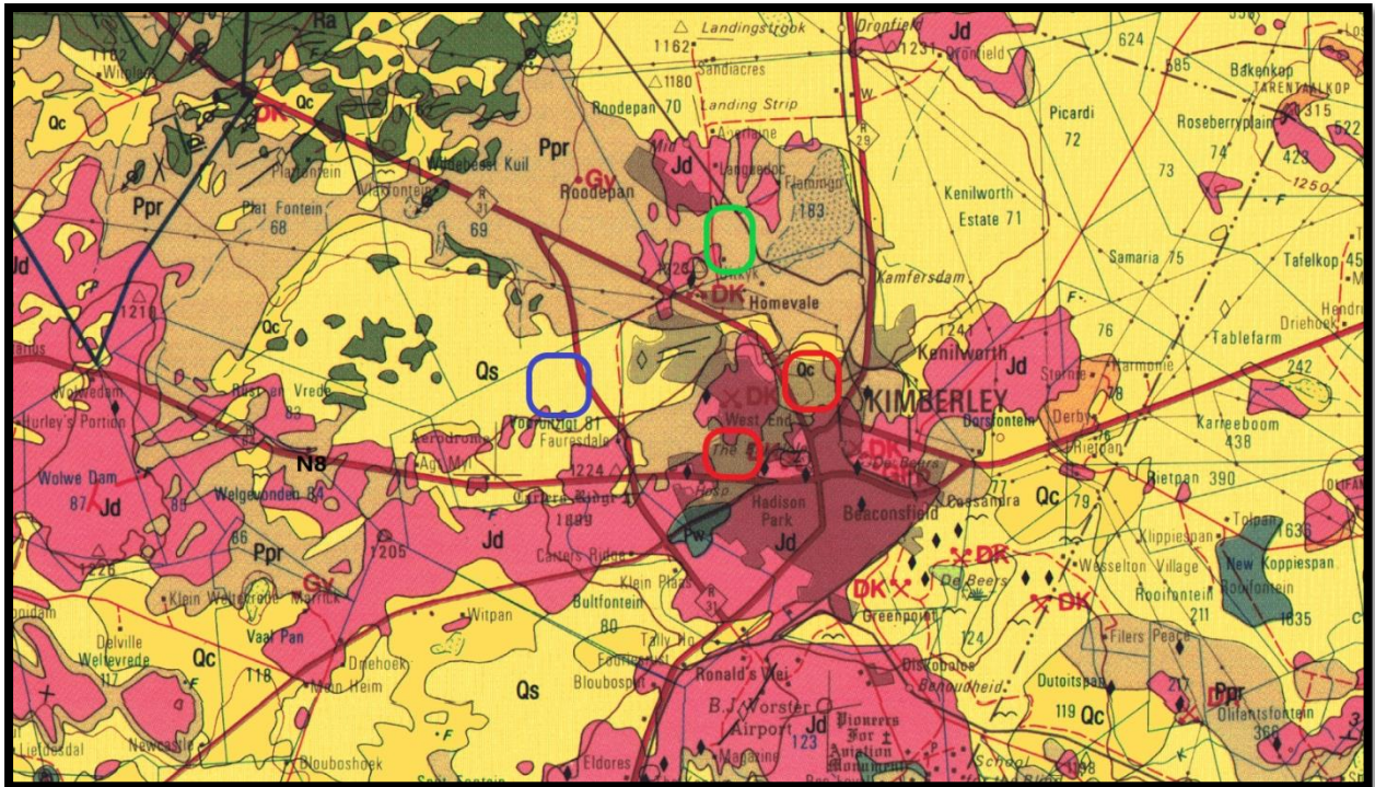
Figure 3: Excerpt of 1:250 000 Geological Map 2824 Kimberley (Bosch and Visser 1994) (1h).
