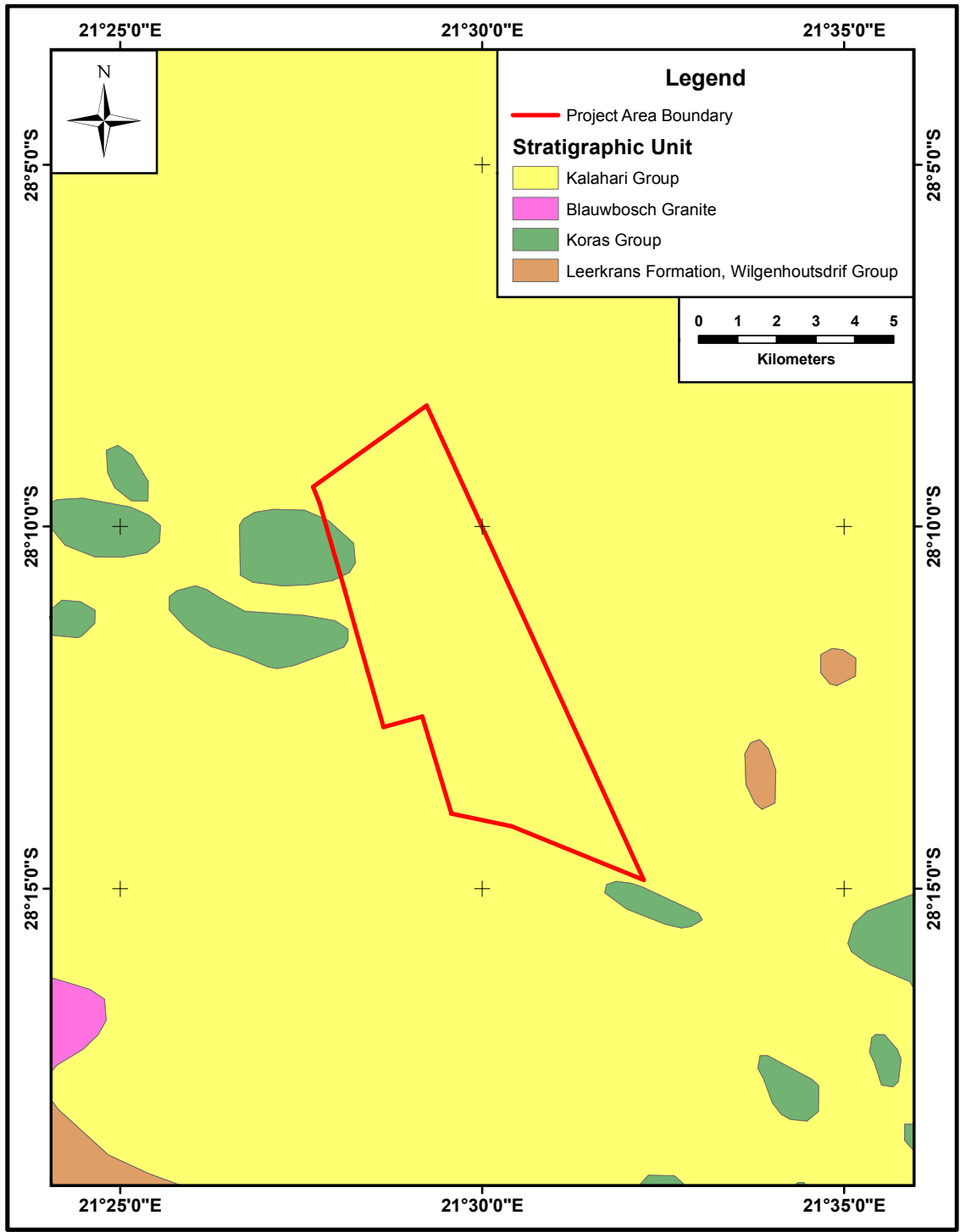
Figure 3: Map of the geology underlying the project area and its surrounding environs.
