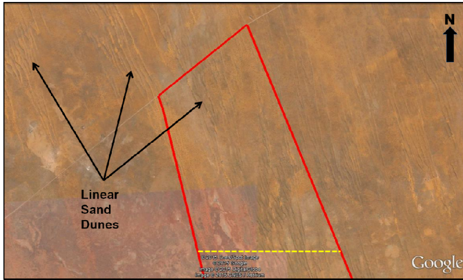
Figure 11: Google earth image of the northern portion of the project area than is presented in the complete view of the project area provided in Figure 4. The extensive cover of Gordonia Formation sand dunes is evident. The yellow, dotted line is in the same position as the similar line in Figure 10.
