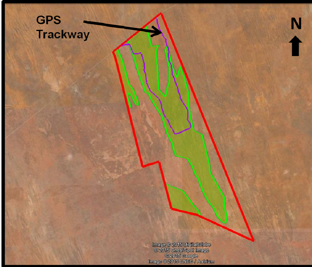
Figure 15: Google earth image of the project area and its immediate environs showing the major sand dune fields present in the area (green polygons) as well as the location of the path of the site investigation (purple line).
