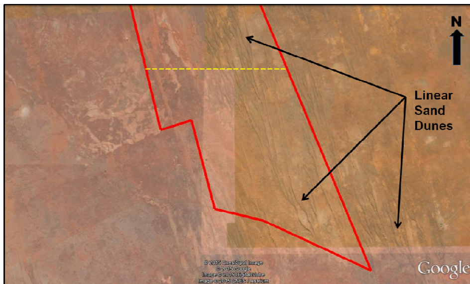
Figure 12: Google earth image of the southern portion of the project area than is presented in the complete view of the project area provided in Figure 4. The extensive cover of Gordonia Formation sand dunes is evident. The yellow, dotted line is in the same position as the similar line in Figure 10.
