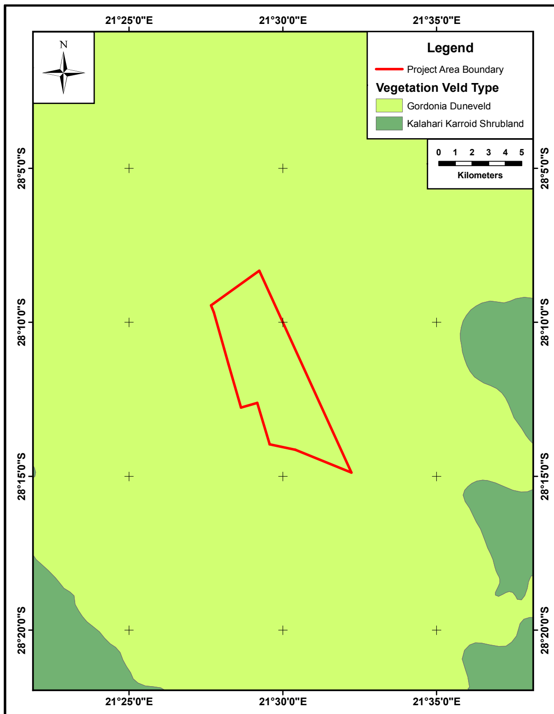
Figure 13: Map of the distribution of the vegetation veld types located within the project area and surrounding environs (after Mucina and Rutherford, 2006).
