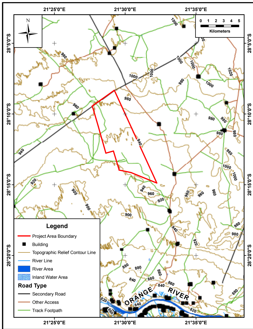
Figure 9: Map of the project area with topographic contours superimposed. It is evident that the project area consists of a flat, featureless landscape. No significant fluvial drainage lines are located within the area, although the Orange River is located several kilometres to the south. The contour interval of the topographic contours is 20 m.
