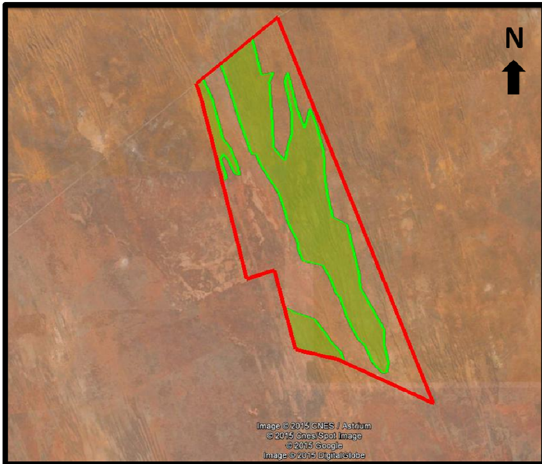
Figure 7: Google earth image of the project area (red polygon) and its immediate environs showing the area of the three main concentrations of linear sand dunes within the project area (green polygons).
