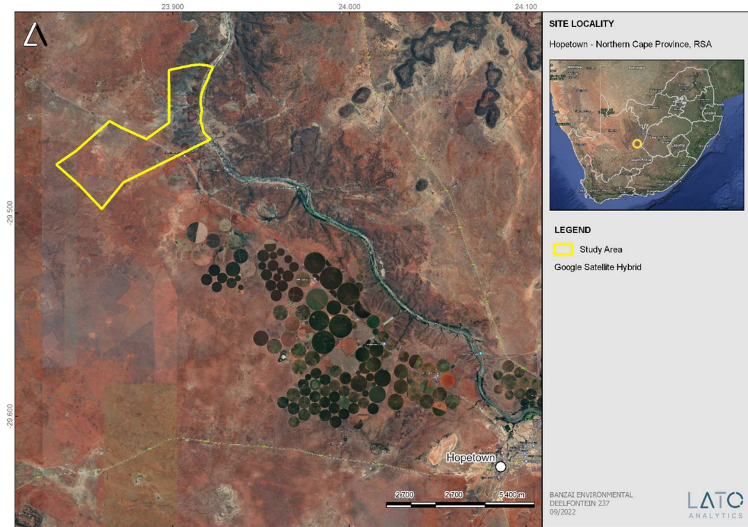
Figure 1: Google Earth (2022) image indicating the regional locality of the proposed Prospecting Right development.
