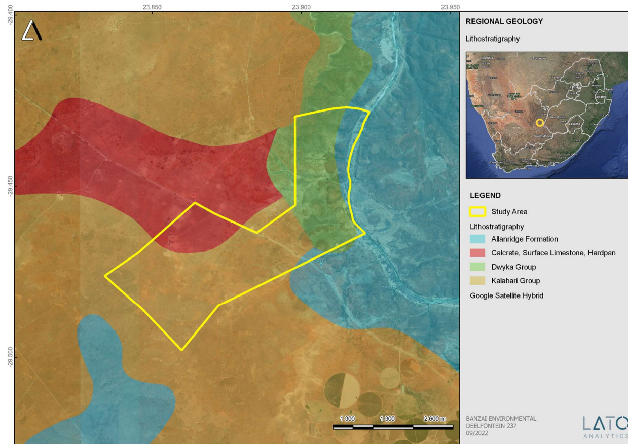
Figure 4: Updated geology (Council for Geosciences, Pretoria) of the proposed development indicates that the development is underlain by the calcrete, surface limestone and Hardpan surface deposits as well as the Kalahari Group, Dwyka Group (Karoo Supergroup) as well as the Allanridge Formation of the Platberg Group Ventersdorp Supergroup.
