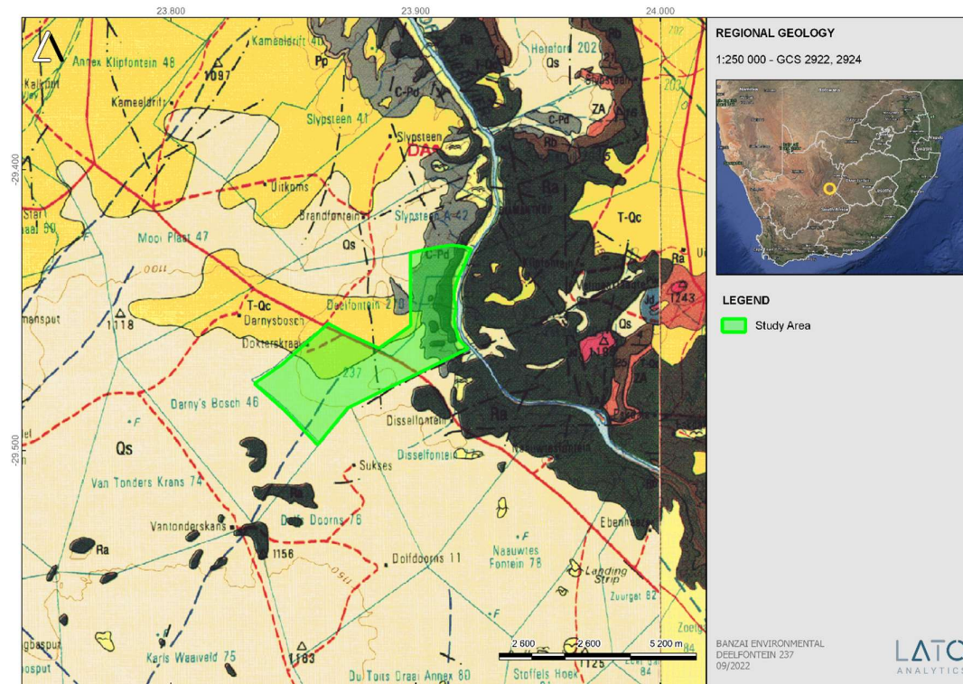
Figure 3: Extract of the 1:250 000 Prieska 2922 (1995) Geological map (Council of Geoscience, Pretoria) indicating the proposed development in green.
