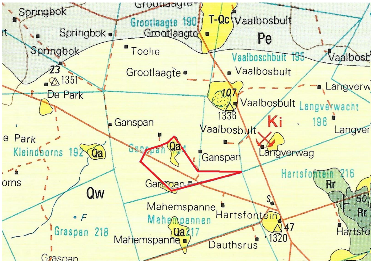
Figure 4: Geology of the study site and surroundings. Adapted from the 2724 CHRISTIANA 1:250 000 Geology Map (Council for Geoscience, 1994)
