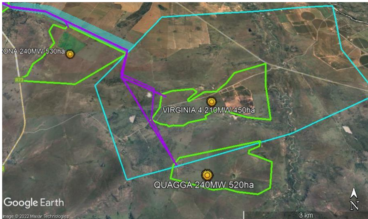
Figure 3: Grid connection of the 132kV line from the solar parks to the approved corridor and Theseus Substation (west).
