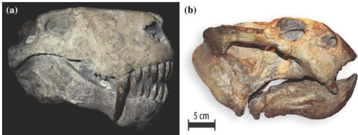
Figure 9: Therapsid skulls representative of two families that went extinct in the Permian: a) flesh eating gorgonopsian, and b) the herbivore dicynodont Daptocephalus (Photos supplied by Bruce Rubidge). In Linol and de Wit (2016) book Preface.
