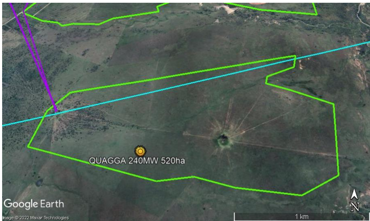
Figure 2: Google Earth map for the proposed Quagga Solar Park (green outline) and the grid connection (purple line).
