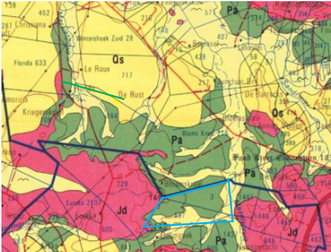
Figure 4: Geological map of the area around the Quagga Solar Park within the blue outline. Abbreviations of the rock types are explained in Table 2. Map enlarged from the Geological Survey 1: 250 000 map 2826 Winburg.
