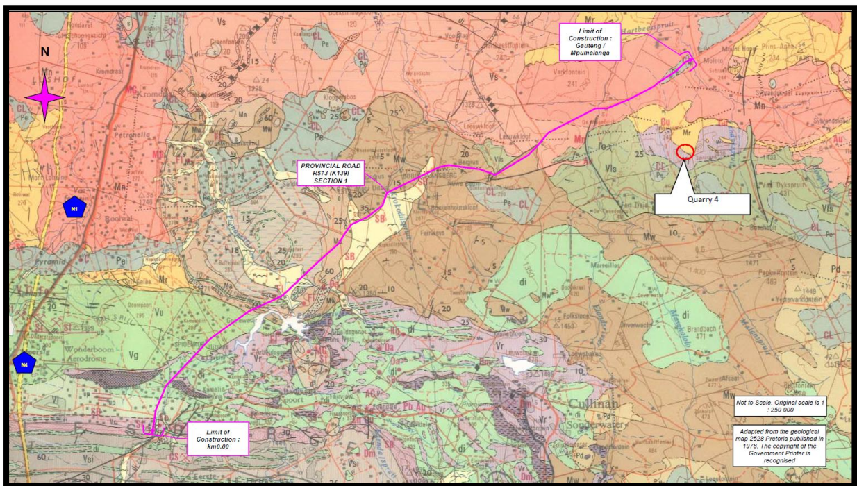
Figure 3: The geology of the development area (Soil Kraft – KBK Engineering).
