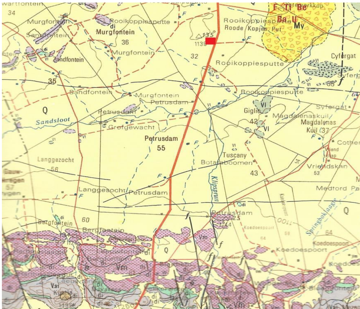
Figure 3: Geological map of the study area and surroundings (adapted from the Rustenburg 2526 1:250 000 Geology Map, Geological Survey, 1981)
