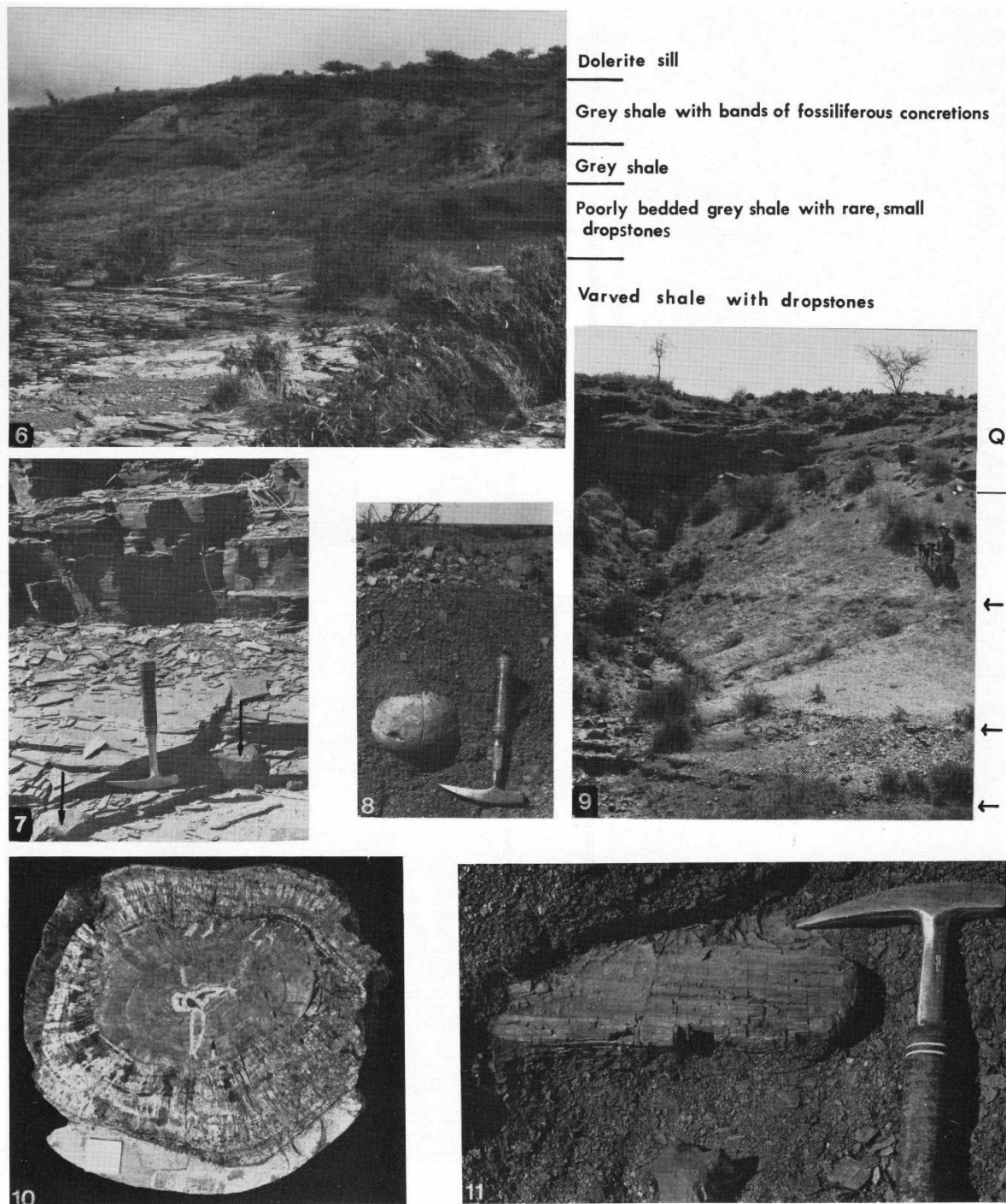
Fig. 6: Blaauw Krantz Site viewed from the east, showing stratigraphy. Fig. 7: Varved shale at Blaauw Krantz. Dropstones to the right and left of hammer head, arrowed. Fig. 8: Concretion in situ at Blaauw Krantz. Fig. 9: Fossiliferous zone at Blaauw Krantz. "Q" indicates Quaternary sediments. The arrows indicate fossiliferous concretion horizons. Fig. 10: Fossil wood from Blaauw Krantz (Specimen BK3). Transverse section ( \times \frac{1}{2} ). Fig. 11: In situ fossil wood at Olie Rivier. Note rounded end.
