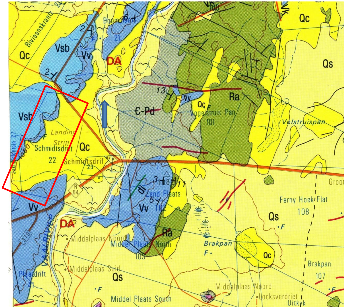
Figure 3: Geological map of the area around Schmidtsdrif town. The location of the proposed project is indicated within the red rectangle. Abbreviations of the rock types are explained in Table 2. Map enlarged from the Geological Survey 1: 250 000 map Kimberley 1993.
