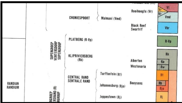
Figure 10: Lithostratigraphic column of the geology of the site (Muntingh 1992).
