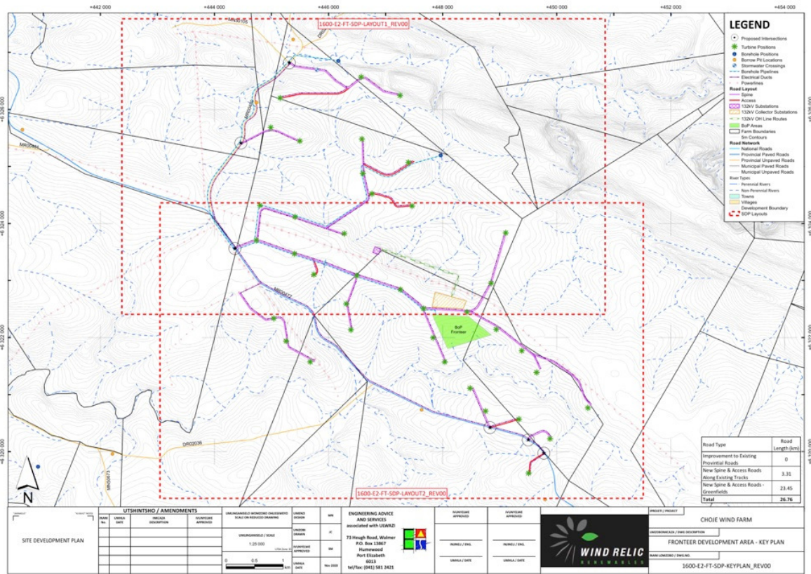
Figure 4: Proposed Frontier WEF development infrastructure (supplied by PGS, 2021)
