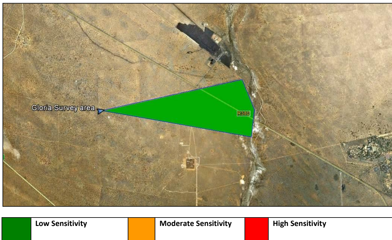
Figure 23 – Palaeontological Sensitivity
