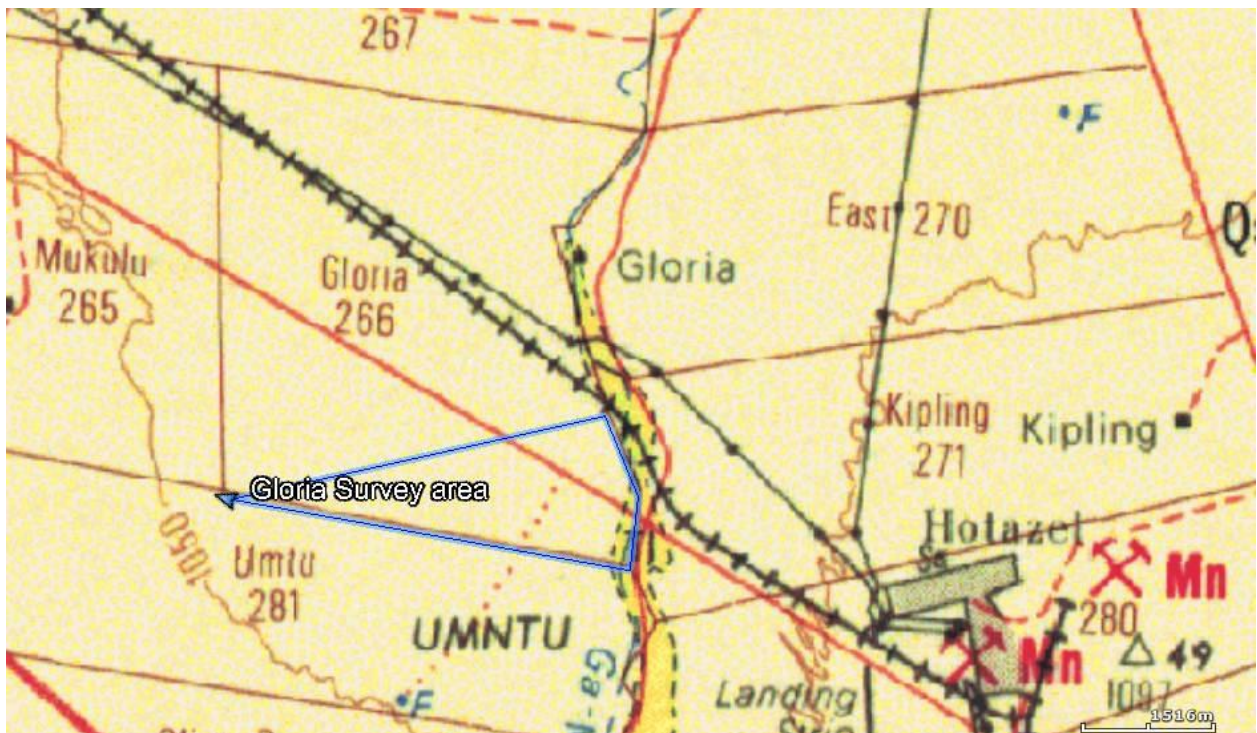
Figure Error! No text of specified style in document..25 Geology of the study area. The entire area is underlain by the Kalahari Formation with a small area in the East underlain by alluvium.
