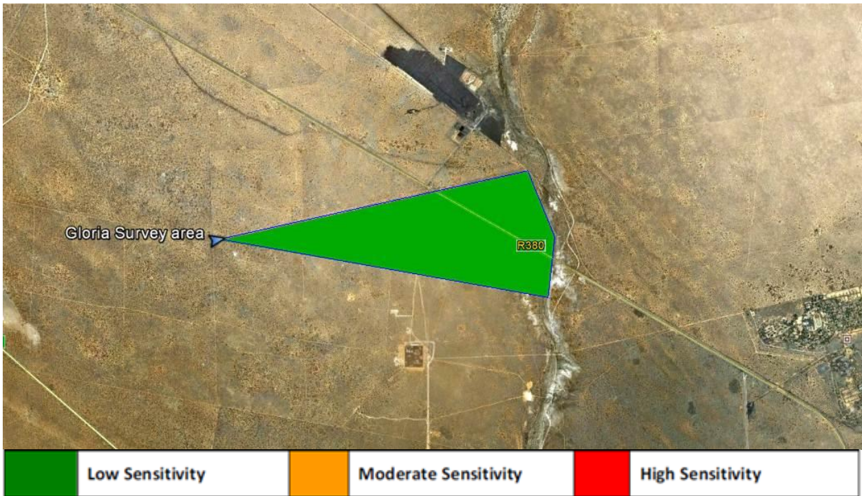
Figure Error! No text of specified style in document..27 Palaeontological sensitivity of the study area
