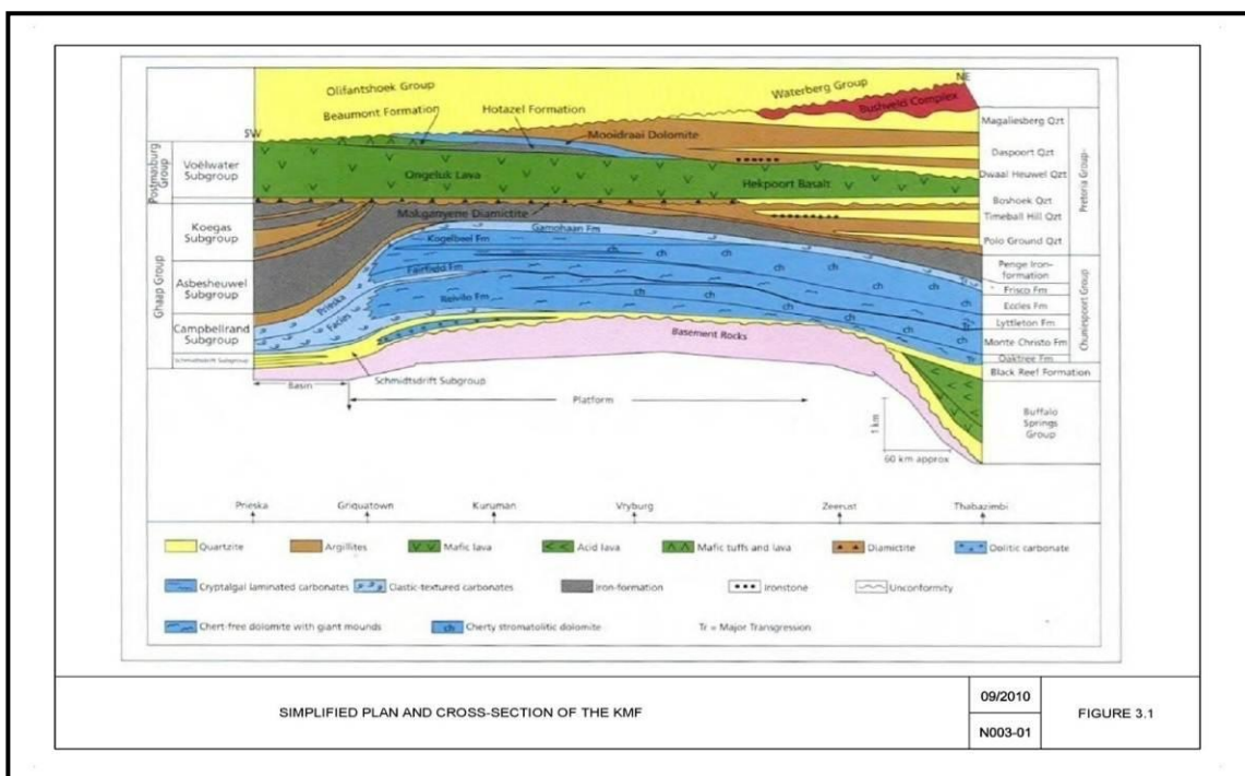
Figure Error! No text of specified style in document..26 Generalised plan of the geology of the Transvaal Supergroup is provided by Beukes (1983) and Van der Merwe (1997).
