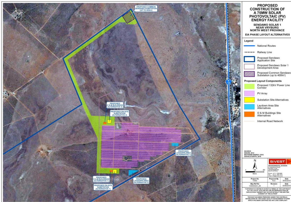
Figure 3 – Sendawo Solar 1 - Layout
