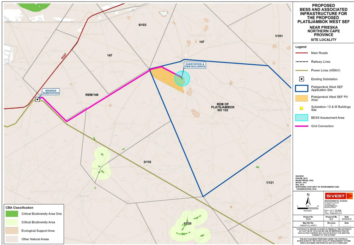
Figure 2: BESS is located on the authorised Platsjambok West Photovoltaic (PV) Energy Facility
